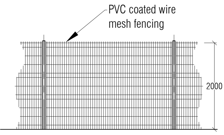
ELEVATION OF 2000mm HIGH BOUNDARY FENCE
