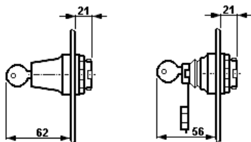
Key-operated switch* -/-pushbutton actuator
