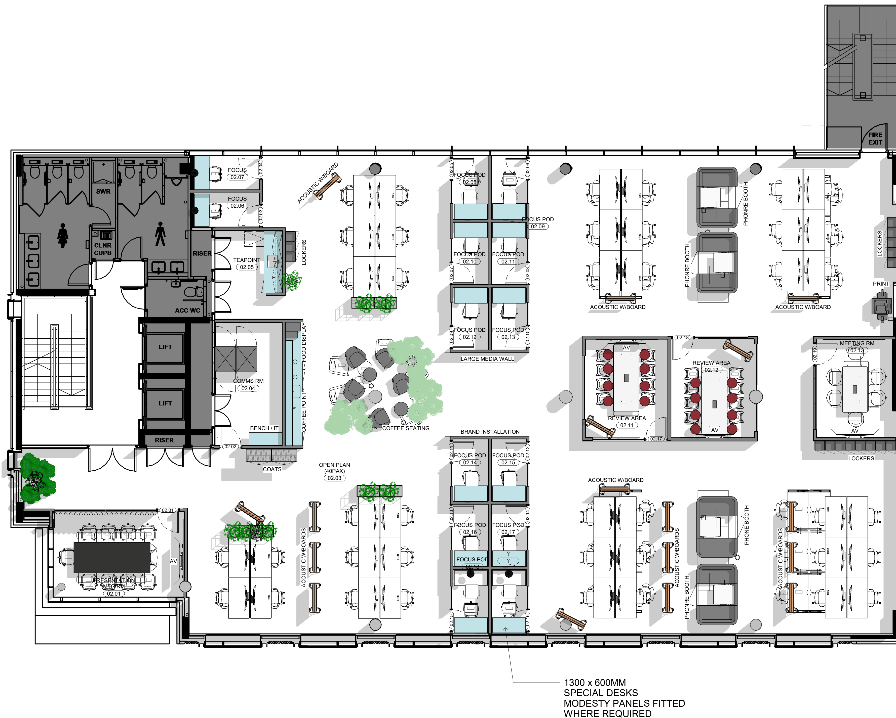
1 GA PLAN - LEVEL 02 (ORANGE FLOOR) 1 : 75
