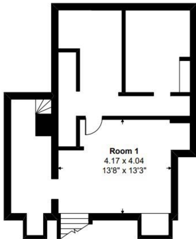
Basement
