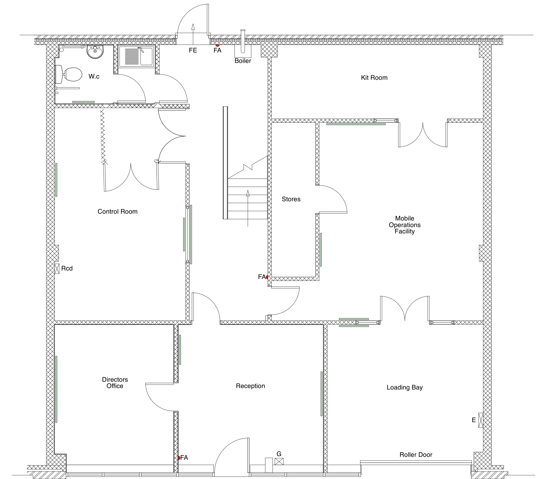
2 Ground Floor Scale: 1:50
