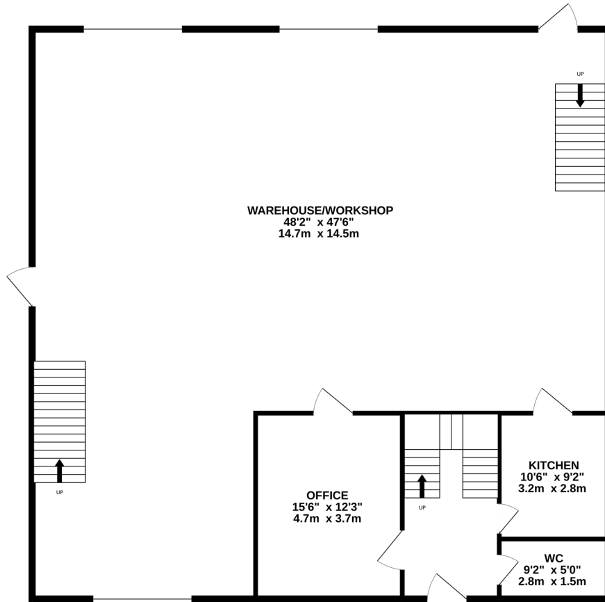
GROUND FLOOR 2307 sq.ft. (214.3 sq.m.) approx.
