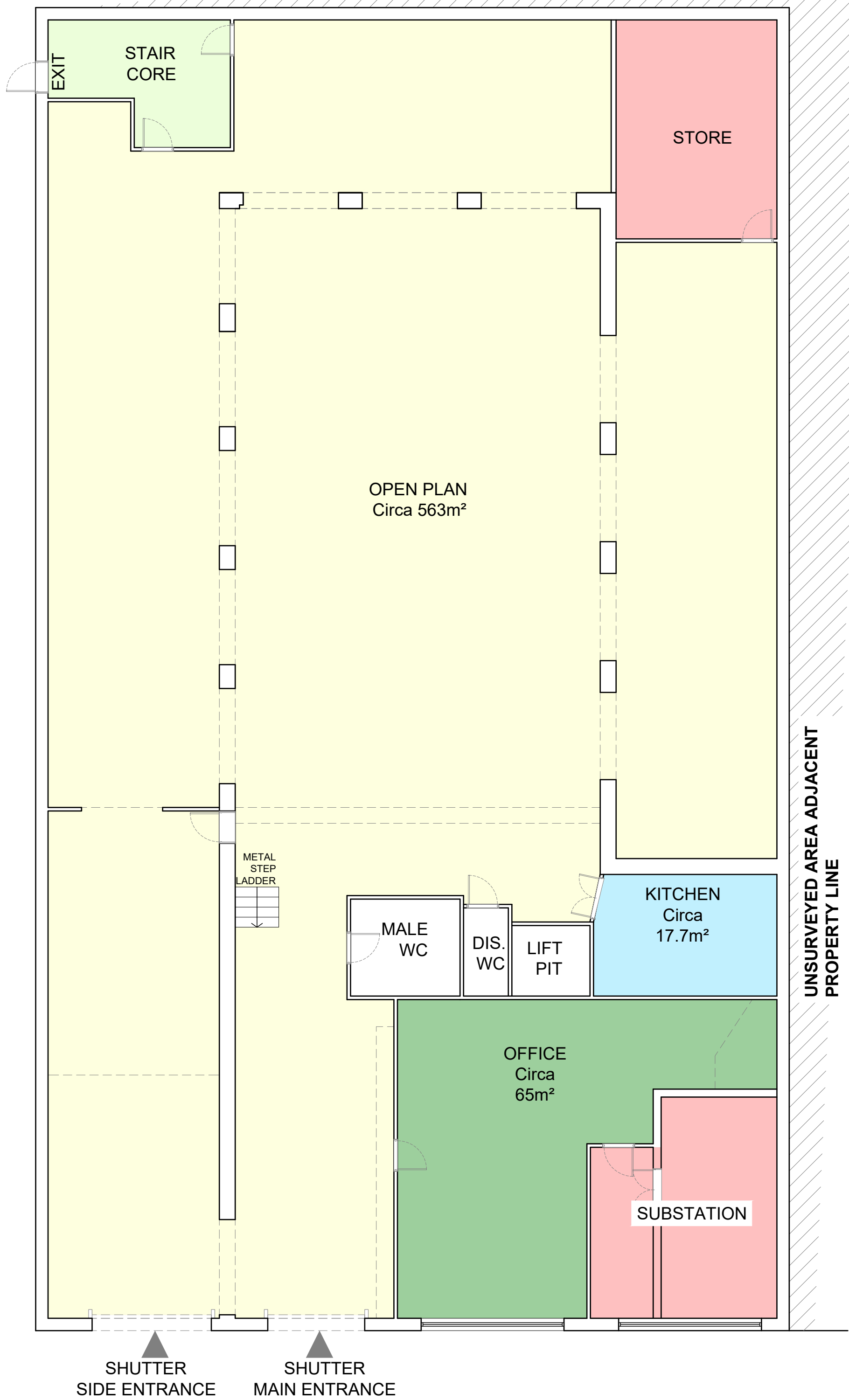
GROUND FLOOR
