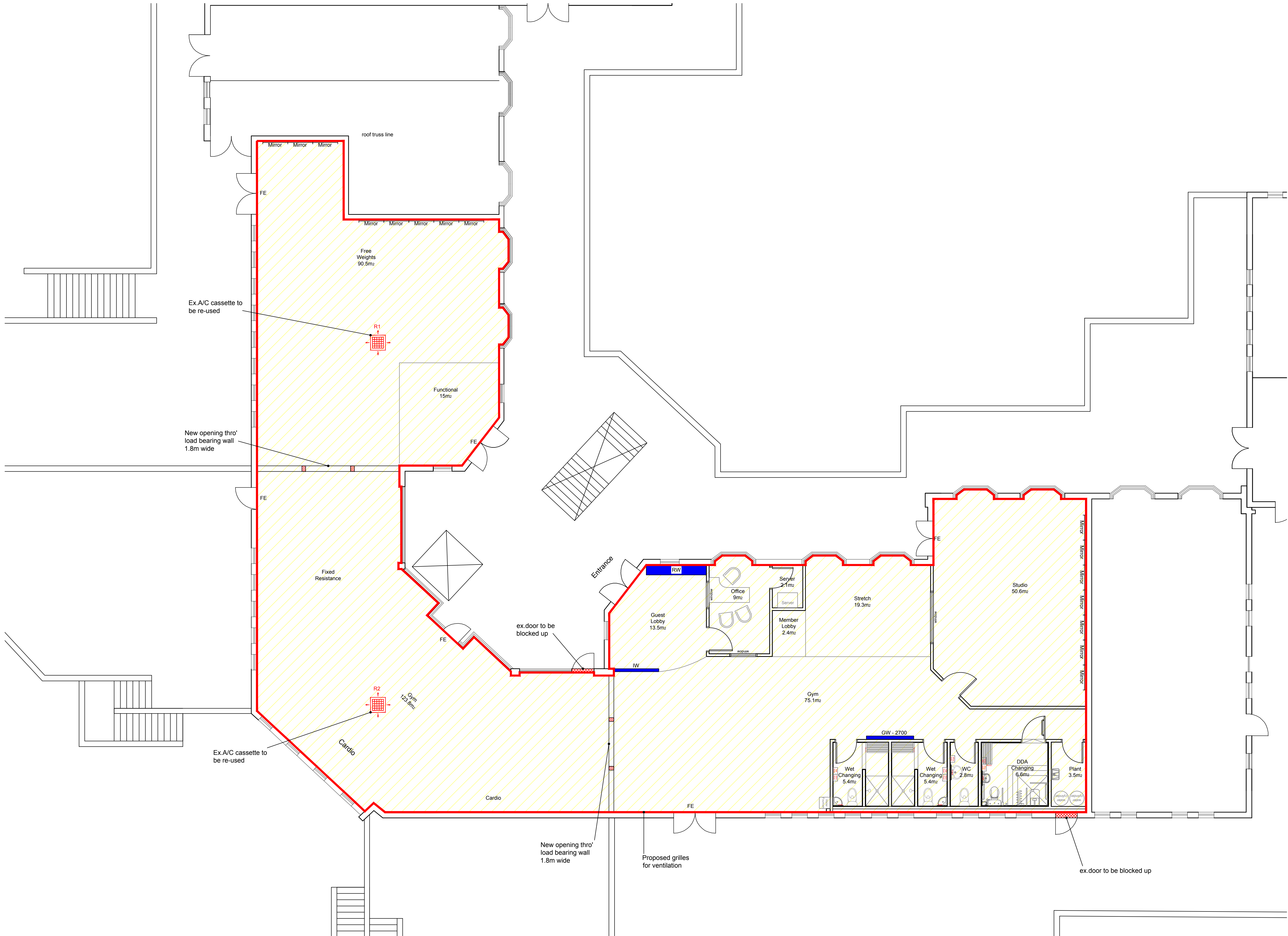
Proposed First Floor Scale 1:100 — Unit Demise
