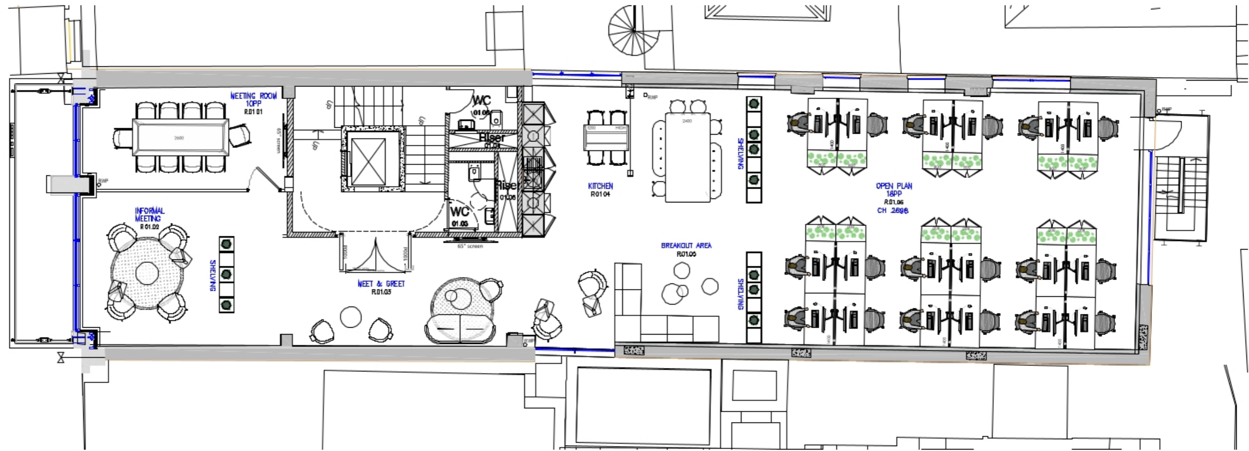
00 LEVEL 01/02/03 - PROPOSED LAYOUT Scale: 1:100 @ A3
