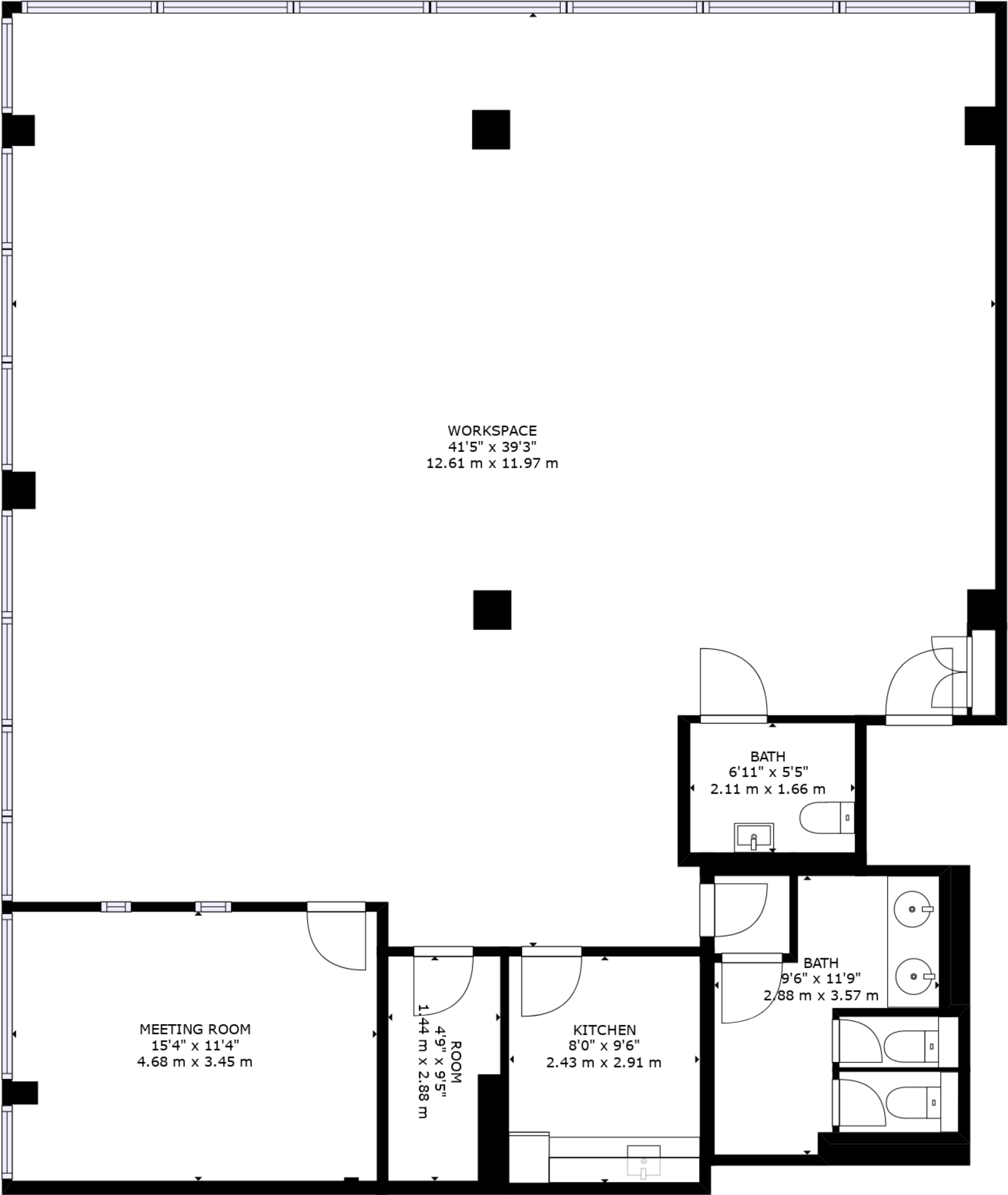
FLOOR 1
