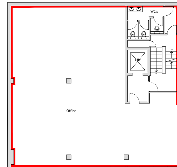
+04 Fourth Floor Plan
