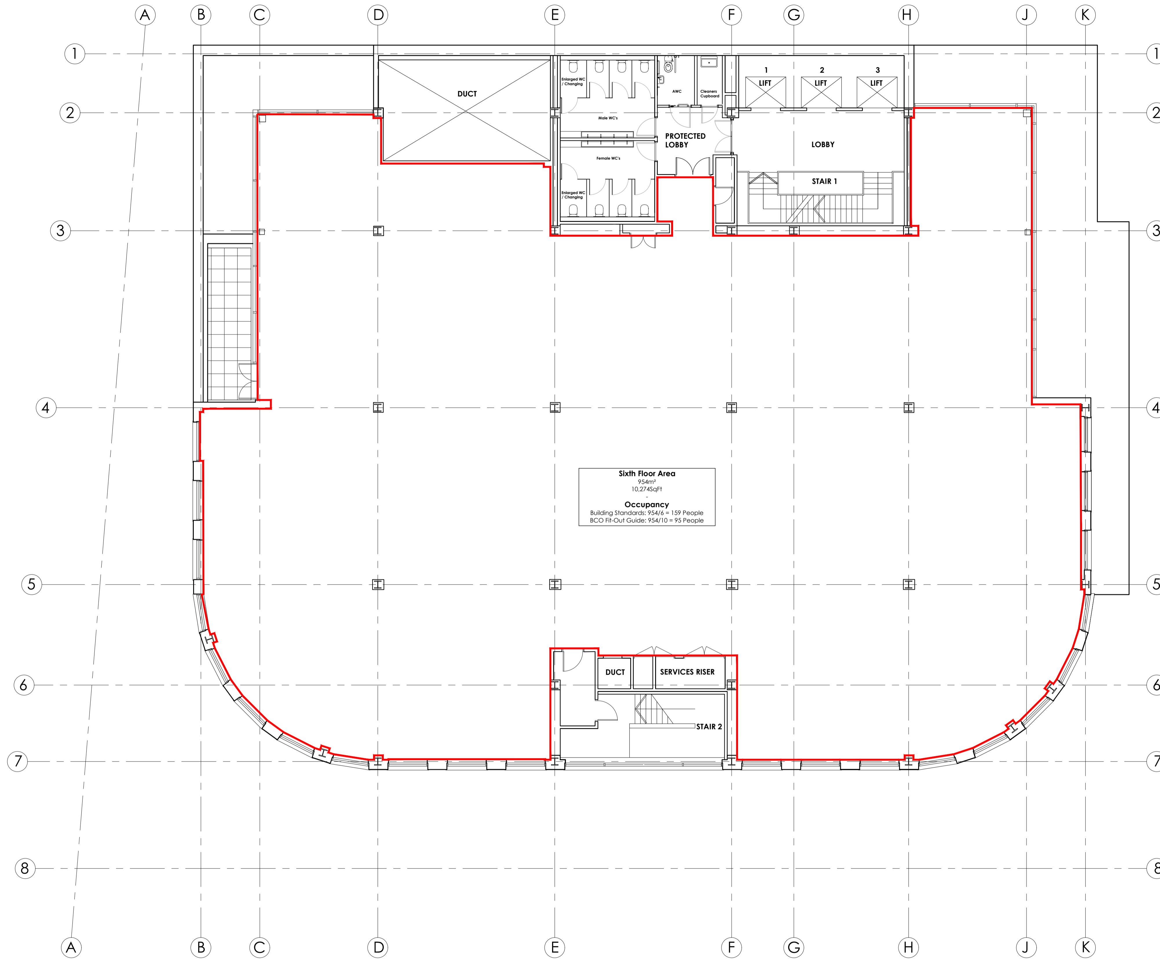
SIXTH FLOOR PLAN AS PROPOSED @ 1:100
