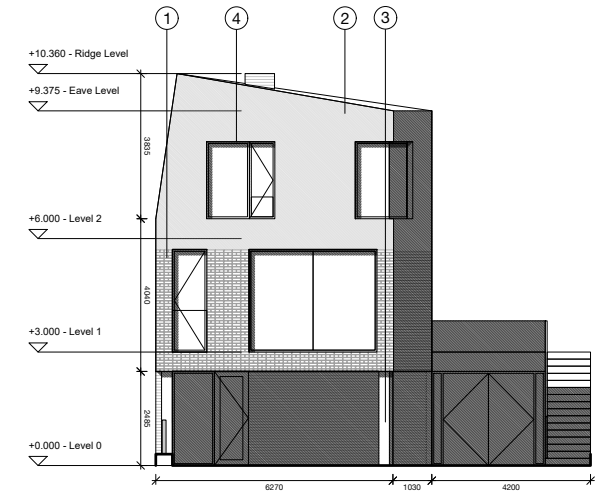
NORTH ELEVATION
