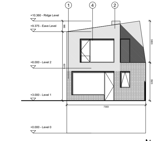
SOUTH ELEVATION
