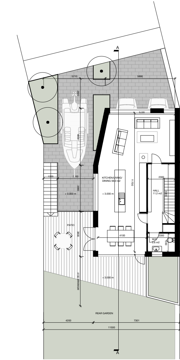
LEVEL 01 PLAN
