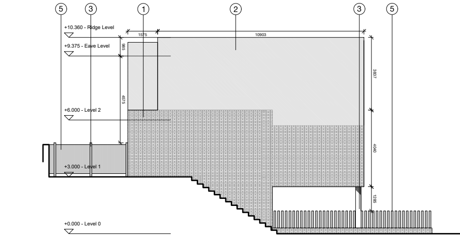
EAST ELEVATION
