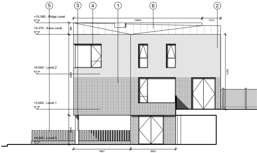
WEST ELEVATION
