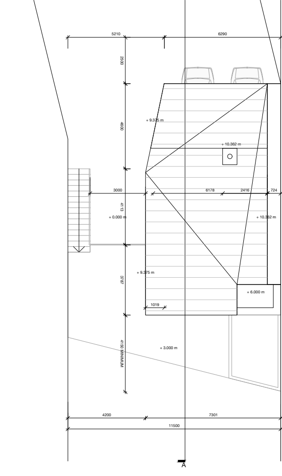
ROOF PLAN
