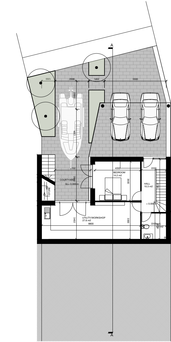
LEVEL 00 PLAN
