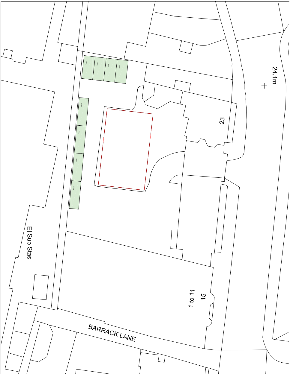
BLOCK PLAN - 1:500
