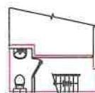
MEZANINE LEVEL PLAN
