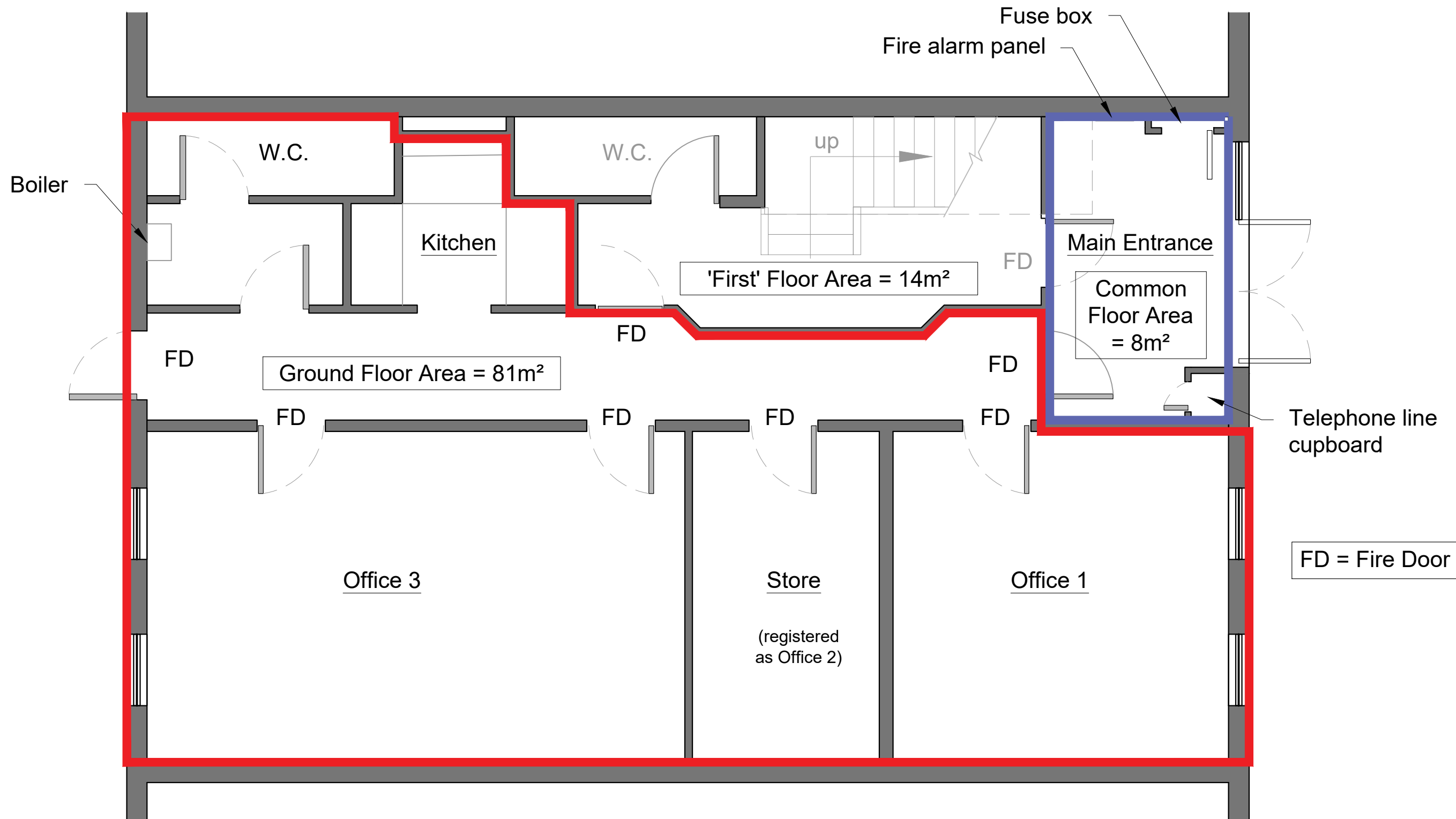
01 Ground Floor Layout
