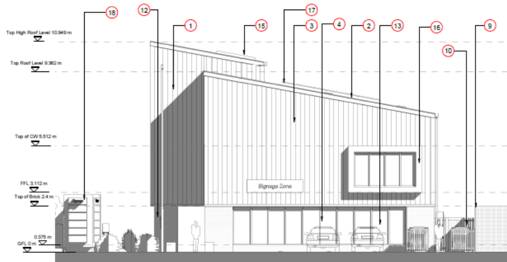
B - WEST ELEVATION - PROPOSED 1 : 100
