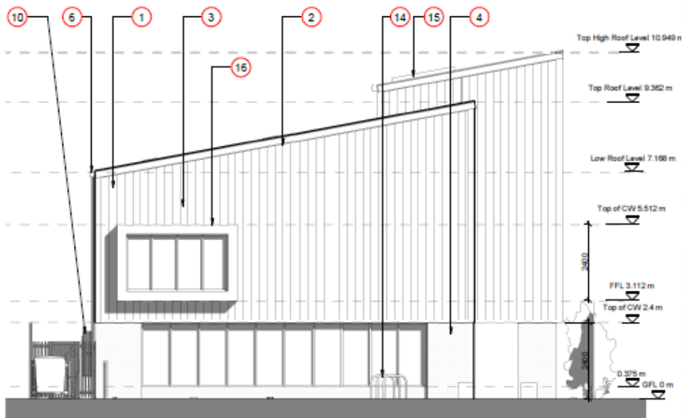
D - EAST ELEVATION - PROPOSED 1:100
