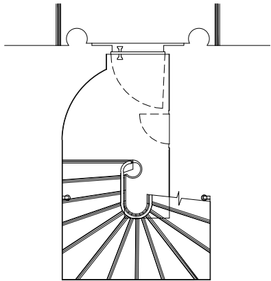
Ground Floor Plan, As Existing, 1:100
