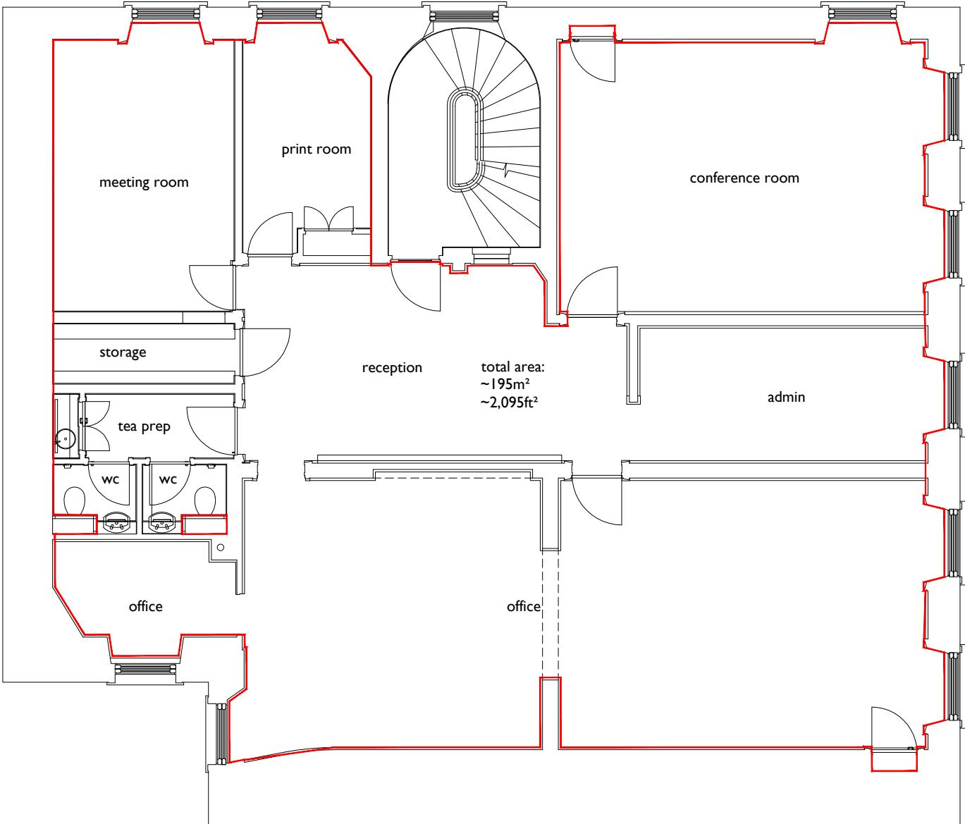
1st Floor Plan, As Existing, 1:100
