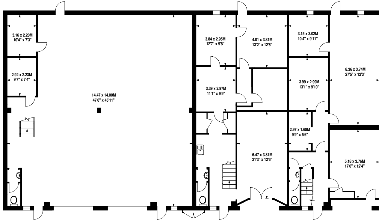
Ground Floor
