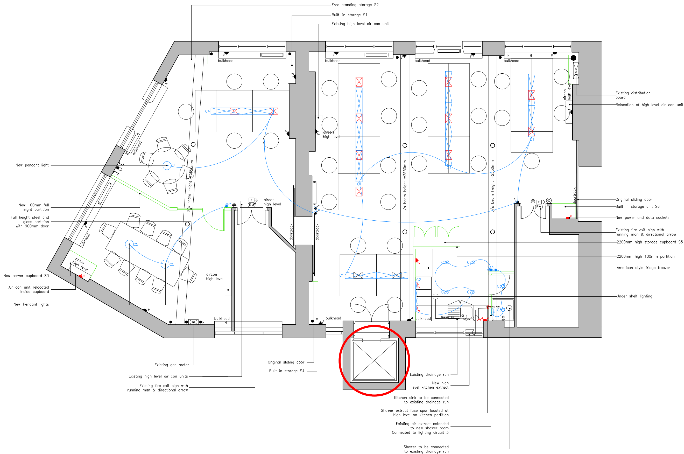
01 PROPOSED OFFICE PLAN 1:75 @ A3
