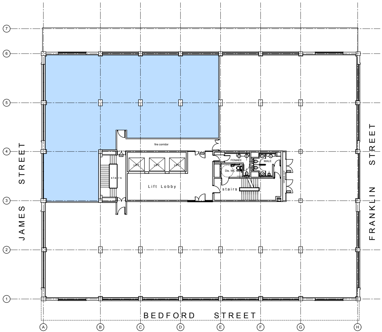
FLOOR PLAN LEVEL 1 SCALE 1:250
