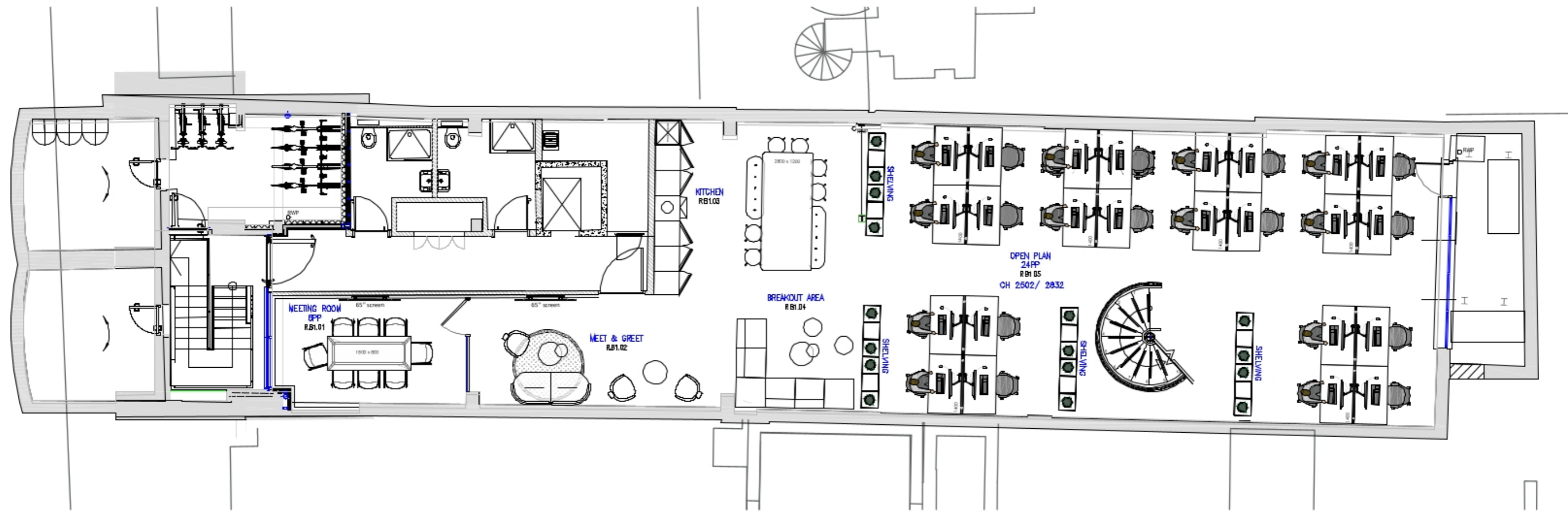
B1 BASEMENT - PROPOSED LAYOUT
