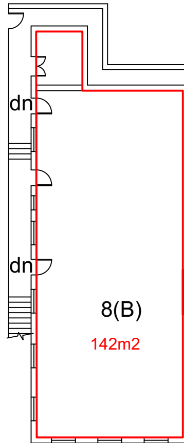
3 First Floor Plan Scale: 1:200
