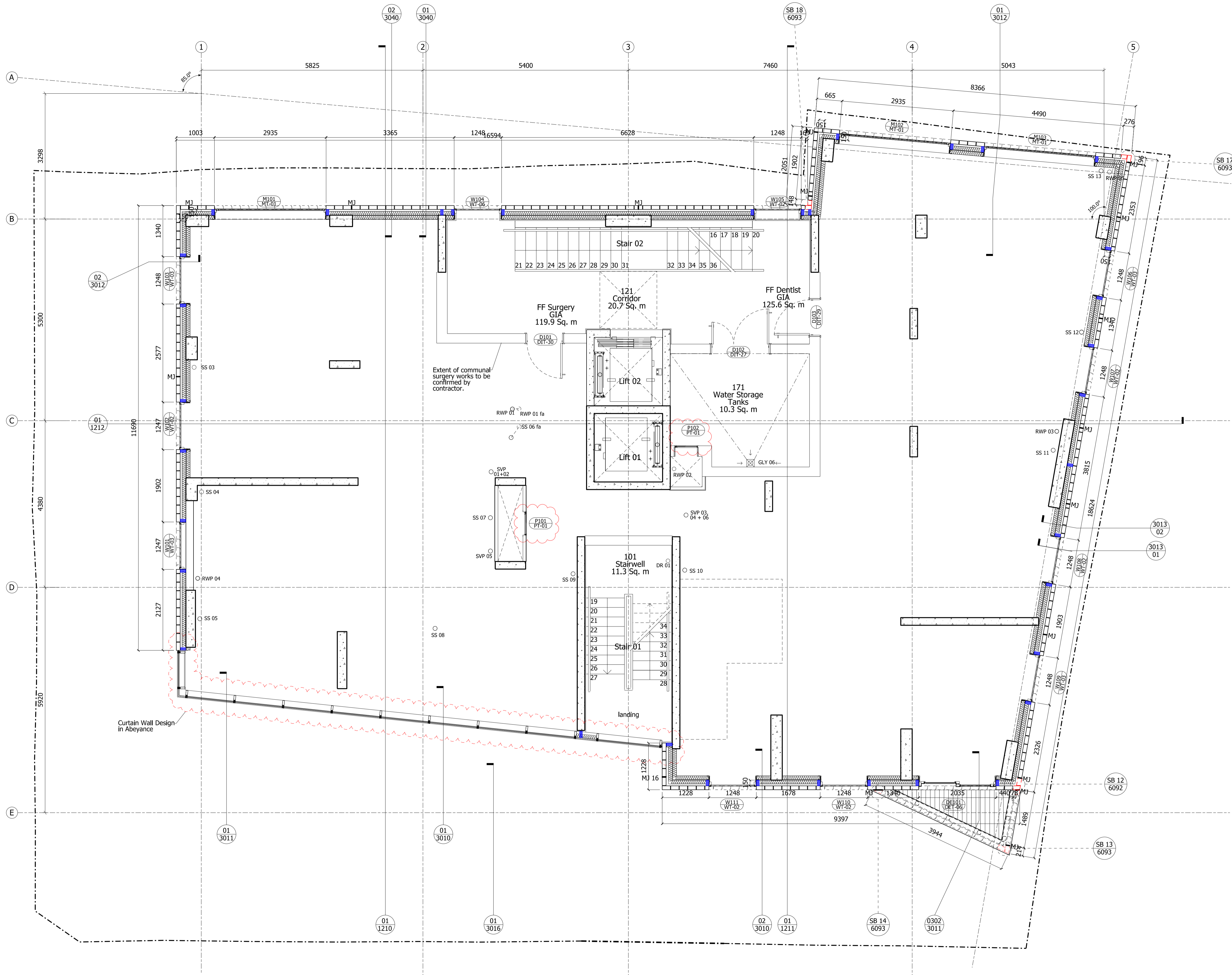
1 First Floor Plan 1:50
