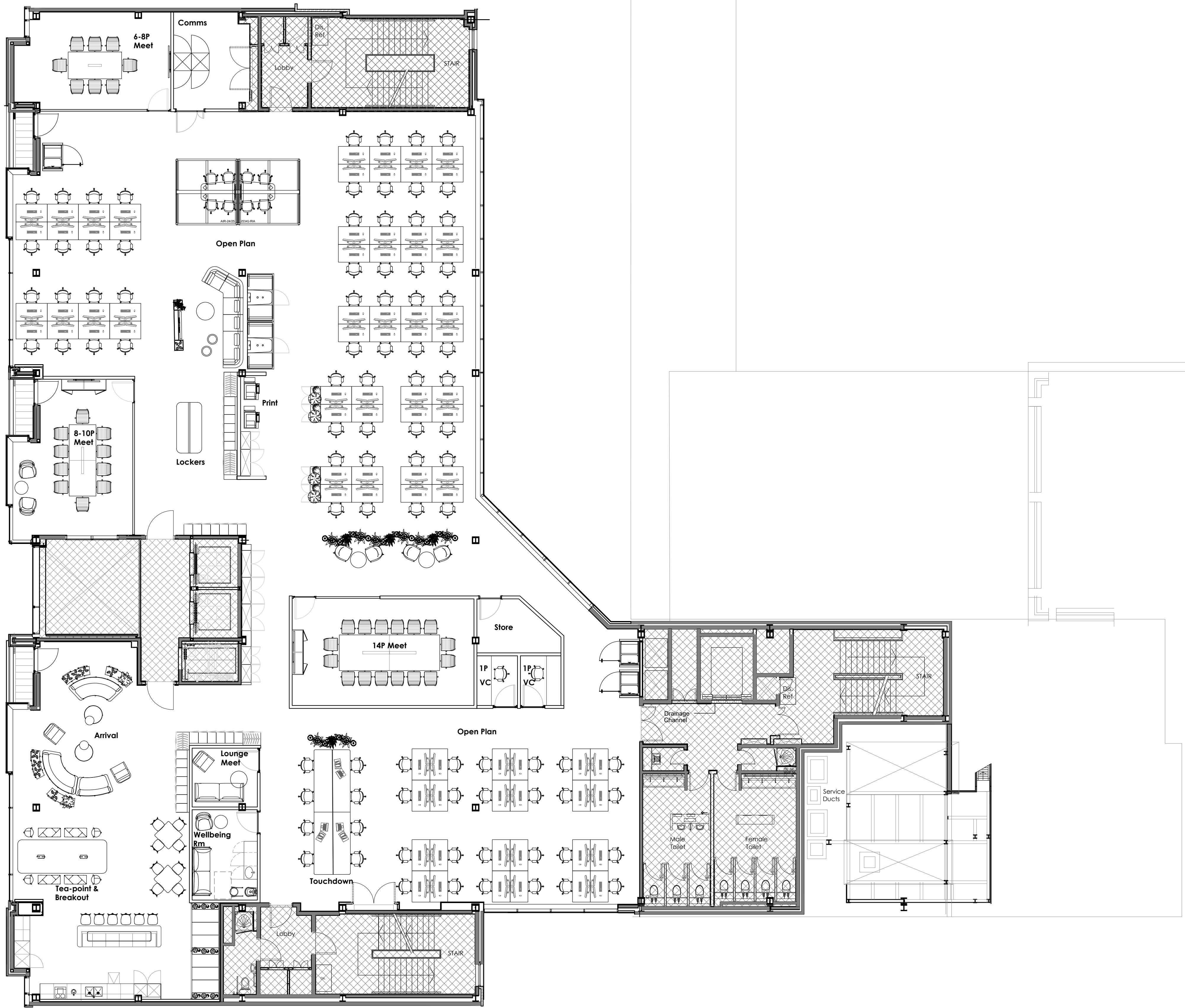
PROPOSED GENERAL ARRANGEMENT PLAN @ 1:100
