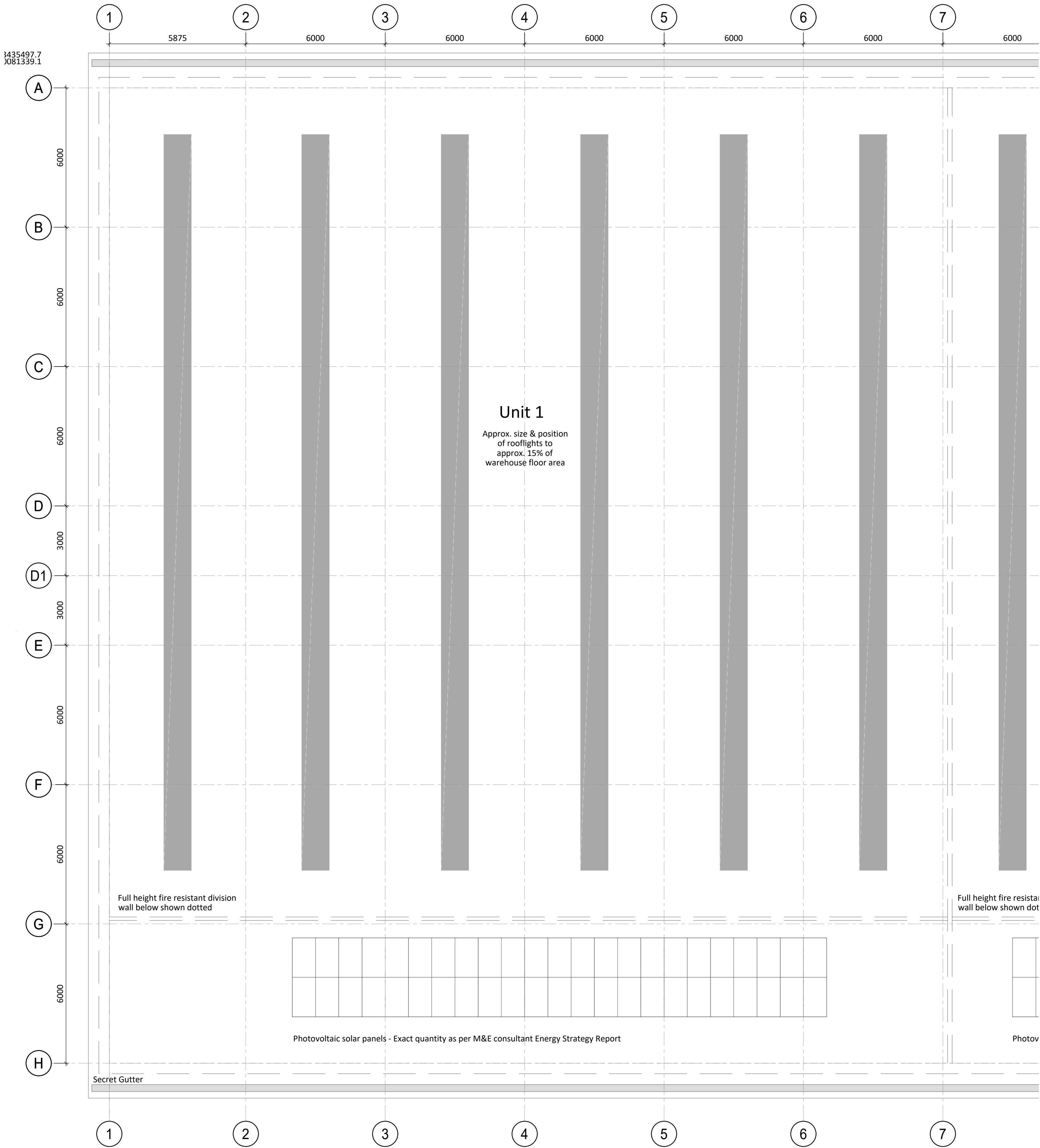
1 Roof Layout 1:100
