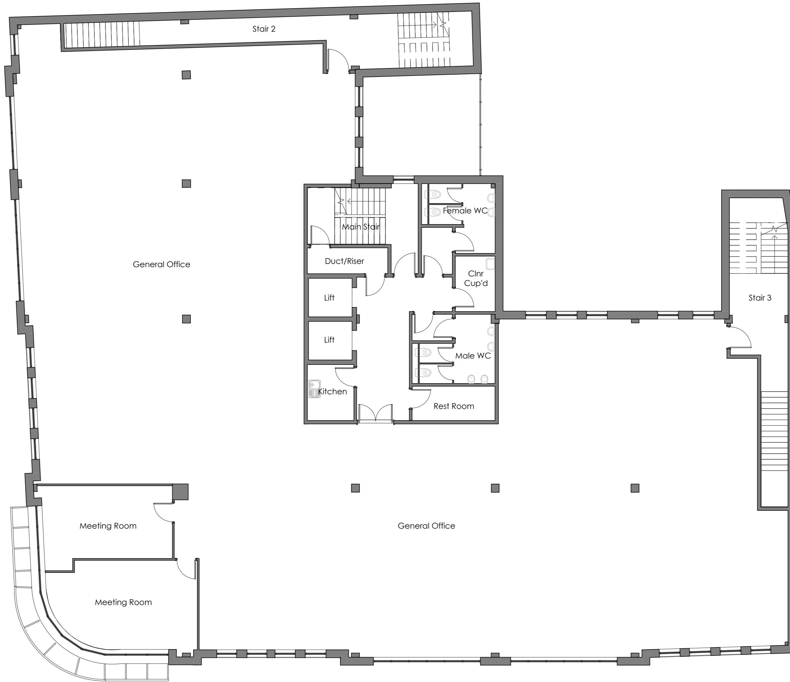
Existing- First Floor Plan 1 : 100
