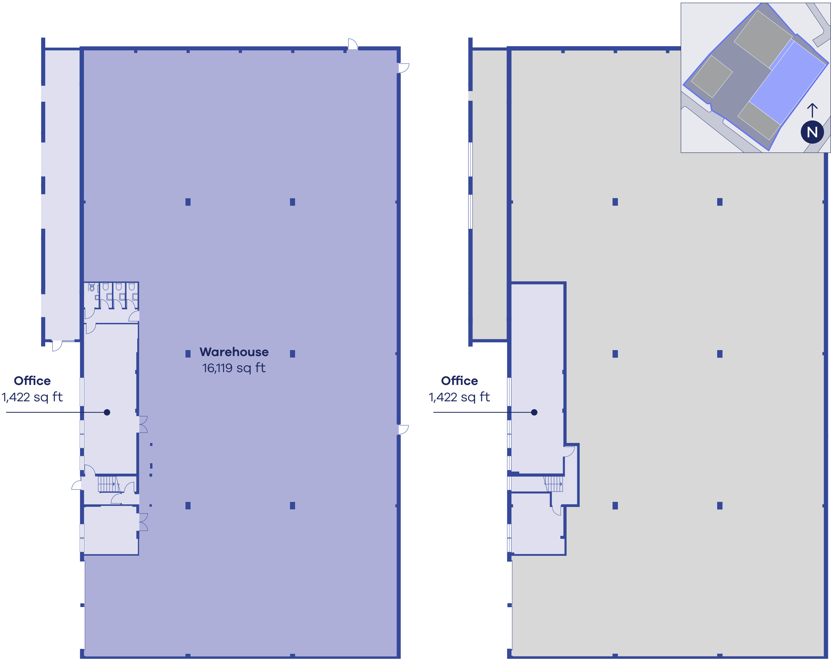
Ground Floor
