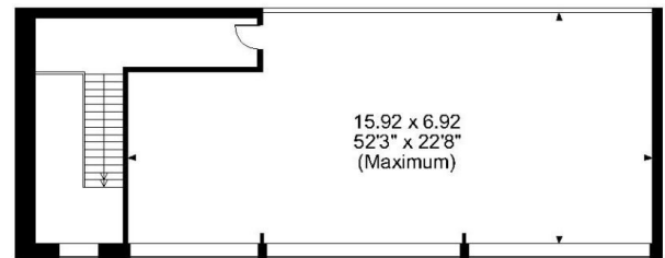
Mezzanine Floor
