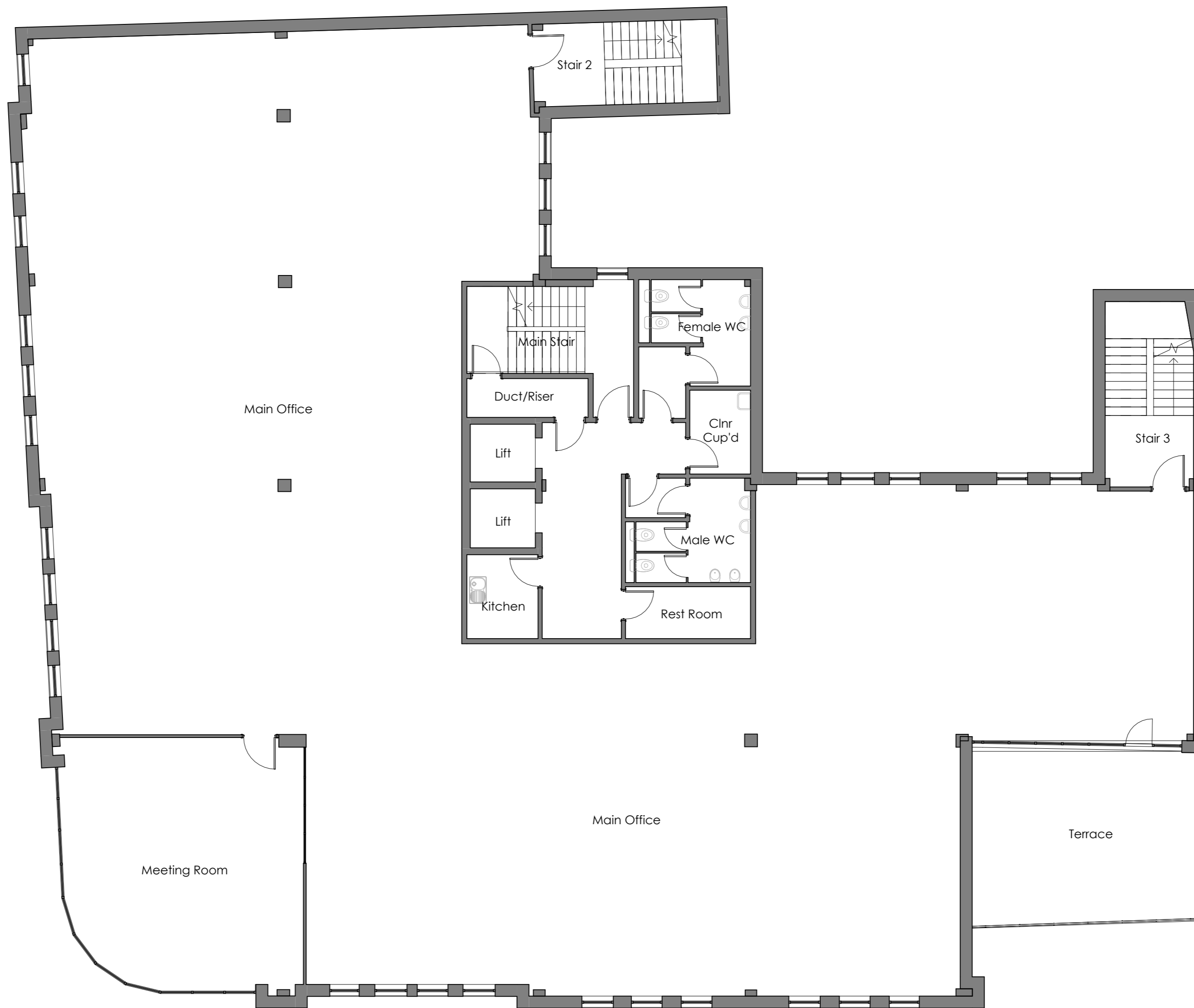
Existing- Third Floor Plan 1 : 100
