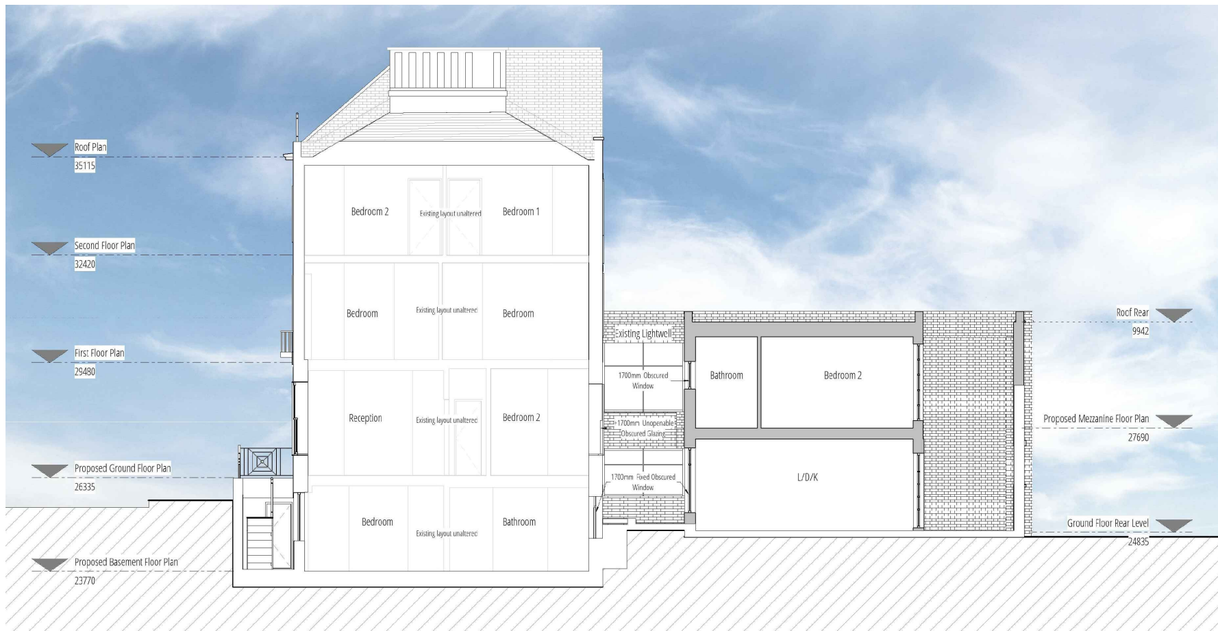
1 Proposed Section DD 1:100
