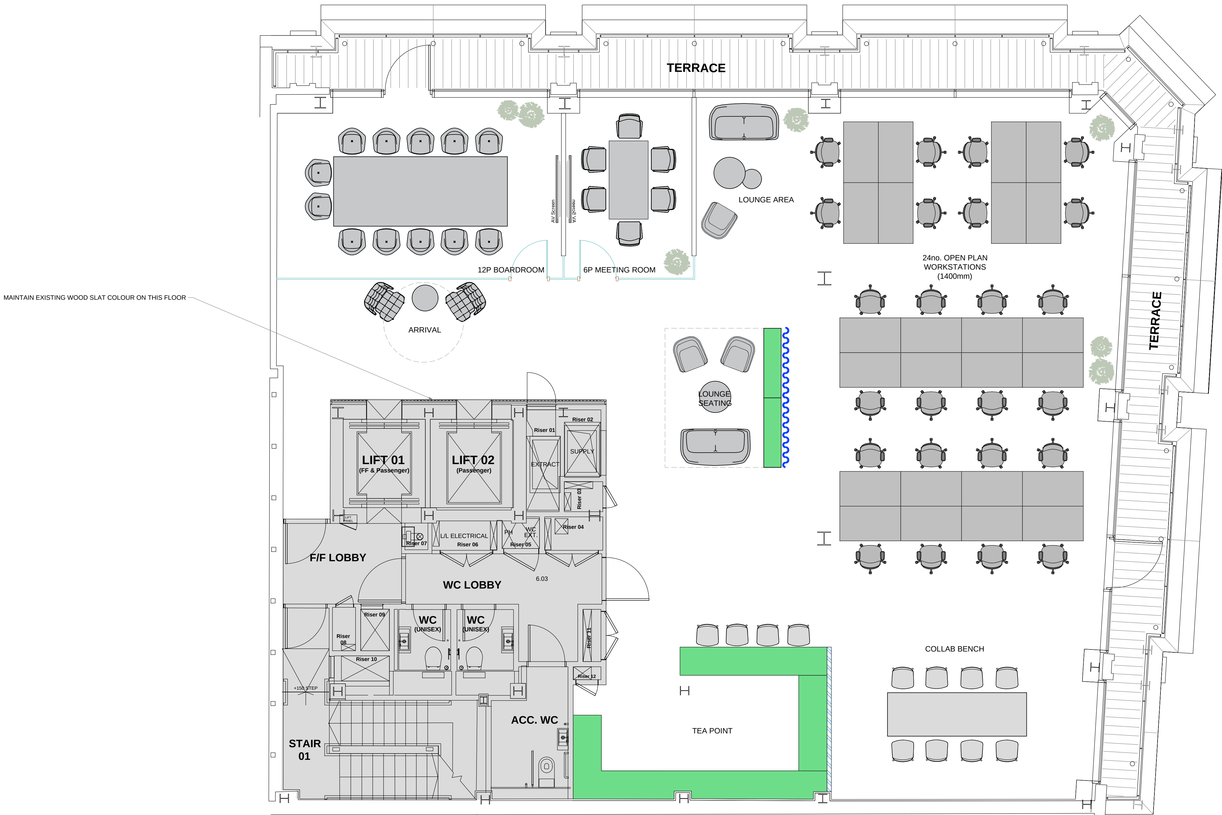
GENERAL ARRANGEMENT - OPTION 1 SCALE 1:50
