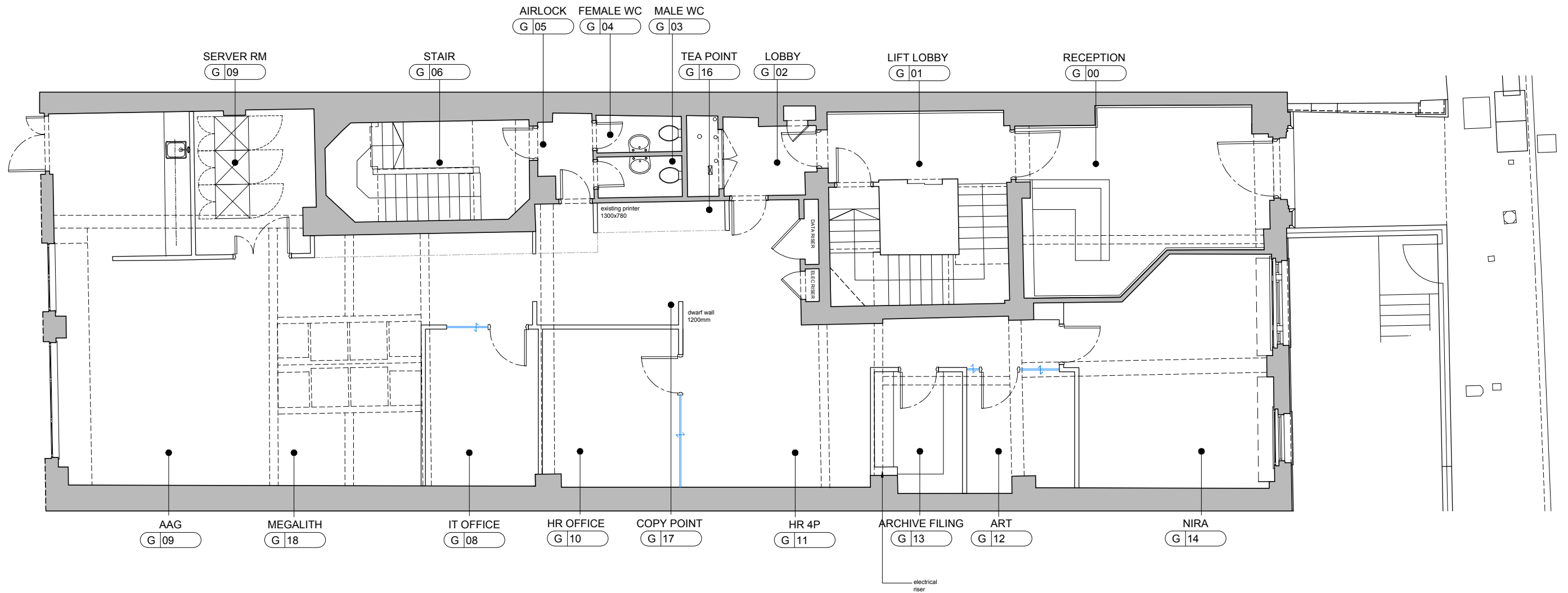
GROUND FLOOR - PARTITION AND DOOR PLAN
