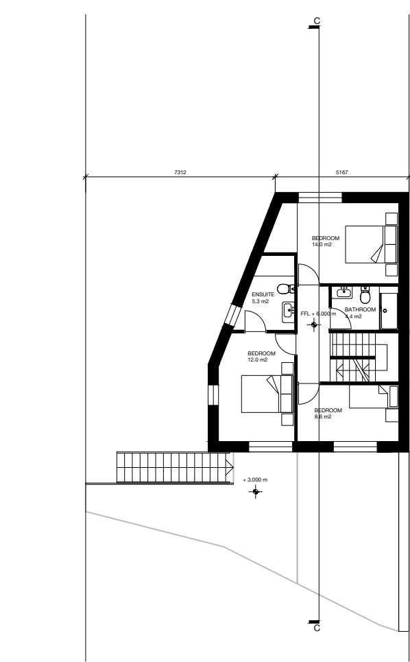
LEVEL 02 PLAN
