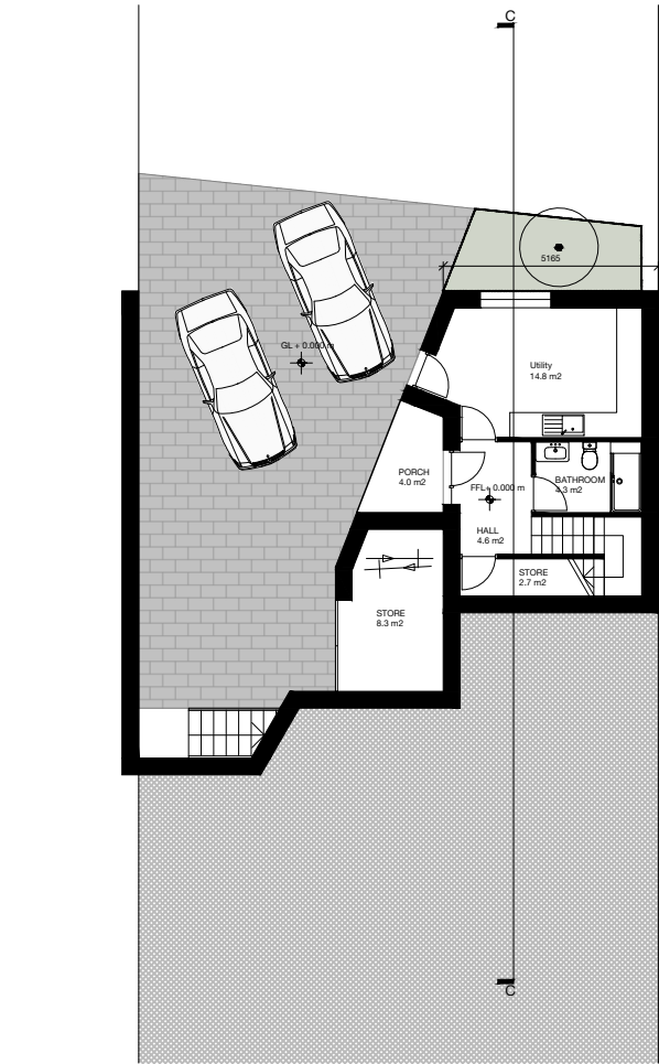
LEVEL 00 PLAN
