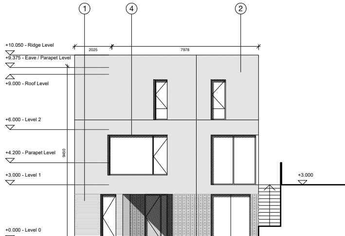
WEST ELEVATION
