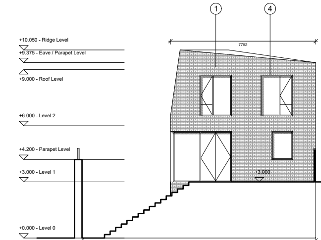
SOUTH ELEVATION
