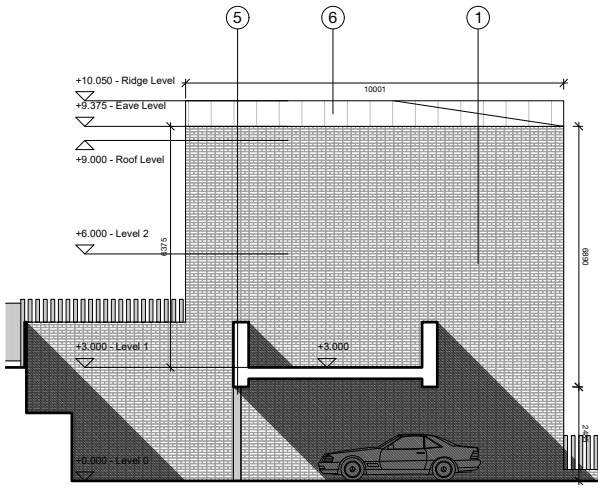
EAST ELEVATION
