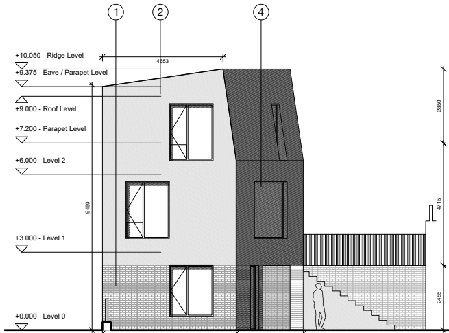
NORTH ELEVATION
