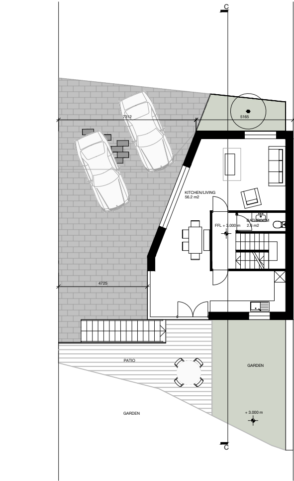
LEVEL 01 PLAN
