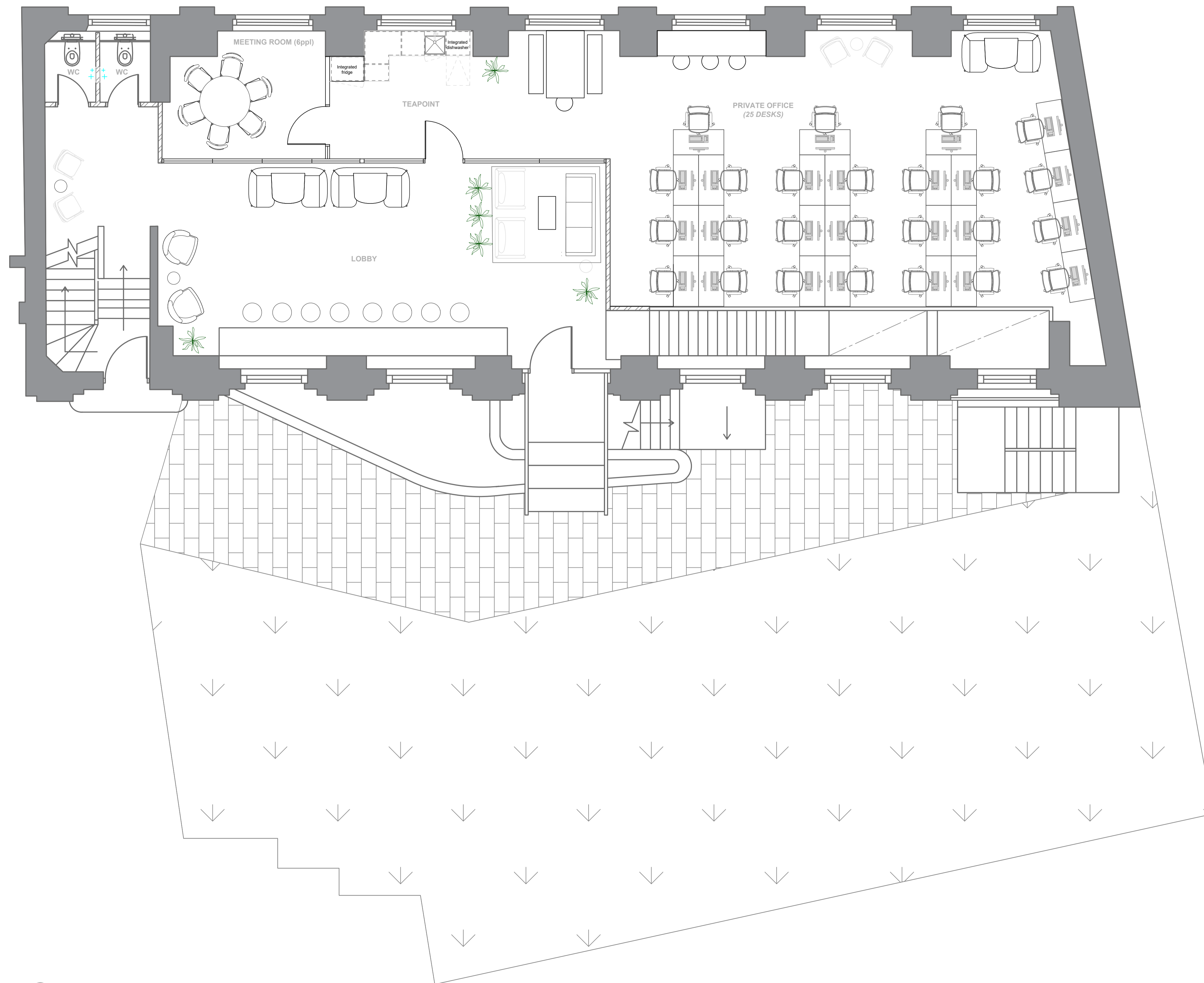
01 GENERAL ARRANGEMENT PLAN SCALE 1:50
