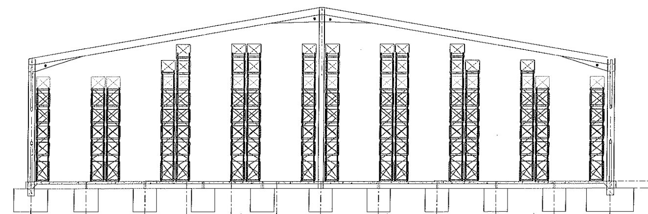
SECTION BB
