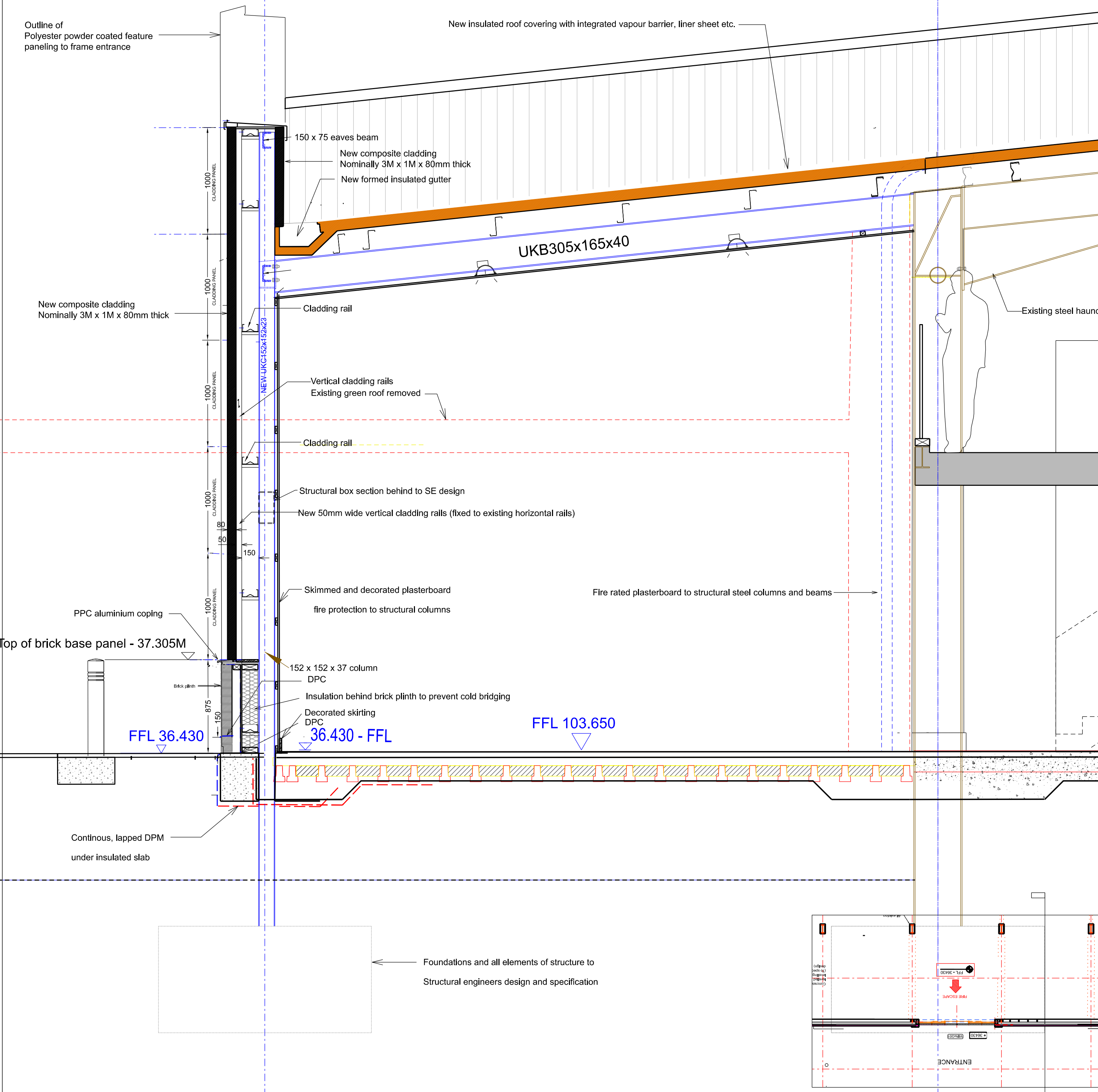
PROPOSED - SECTION A-A THROUGH CLADDING - UNIT 3
