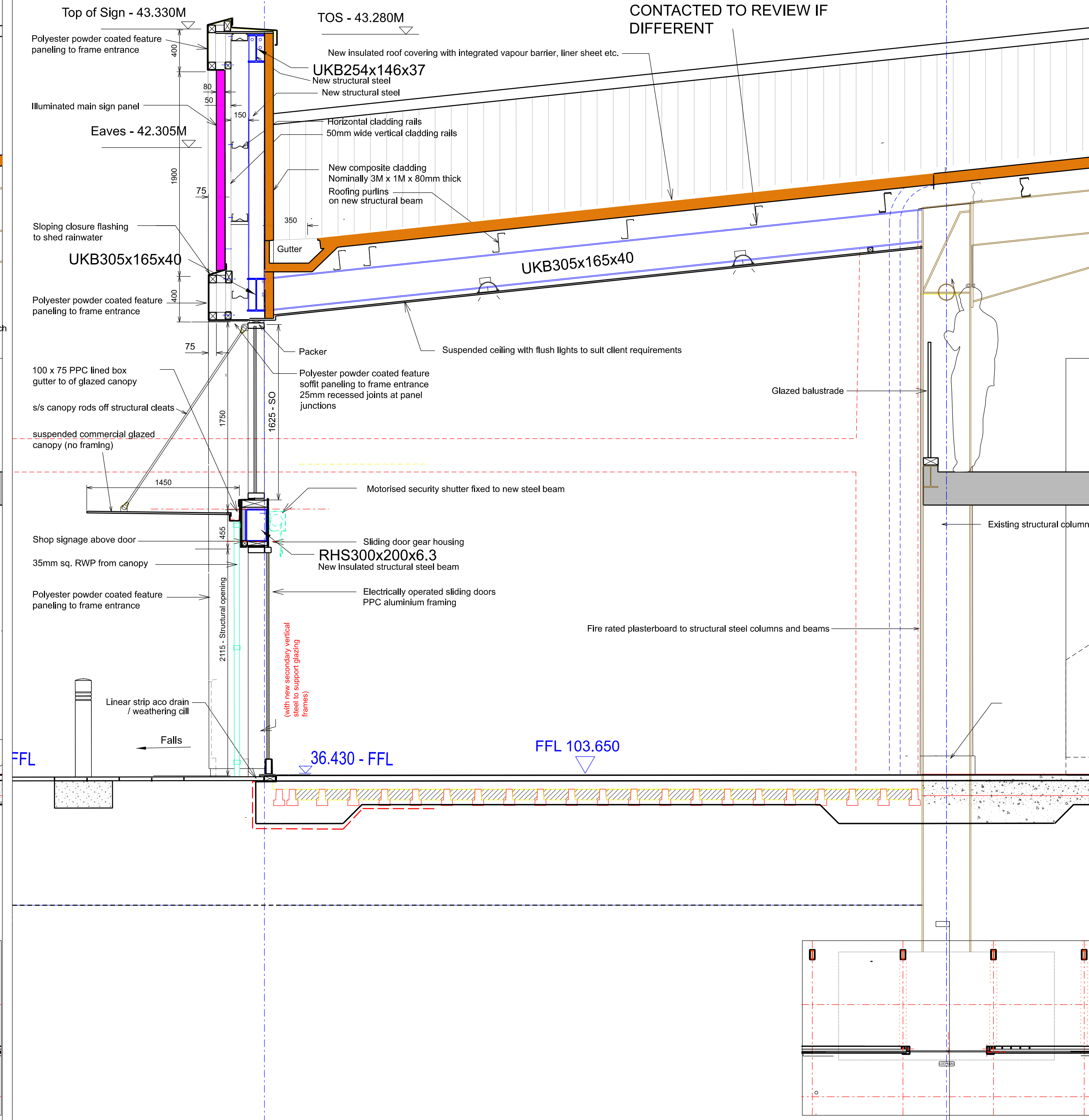
PROPOSED - SECTION B-B THROUGH MAIN ENTRANCE - UNIT 3
