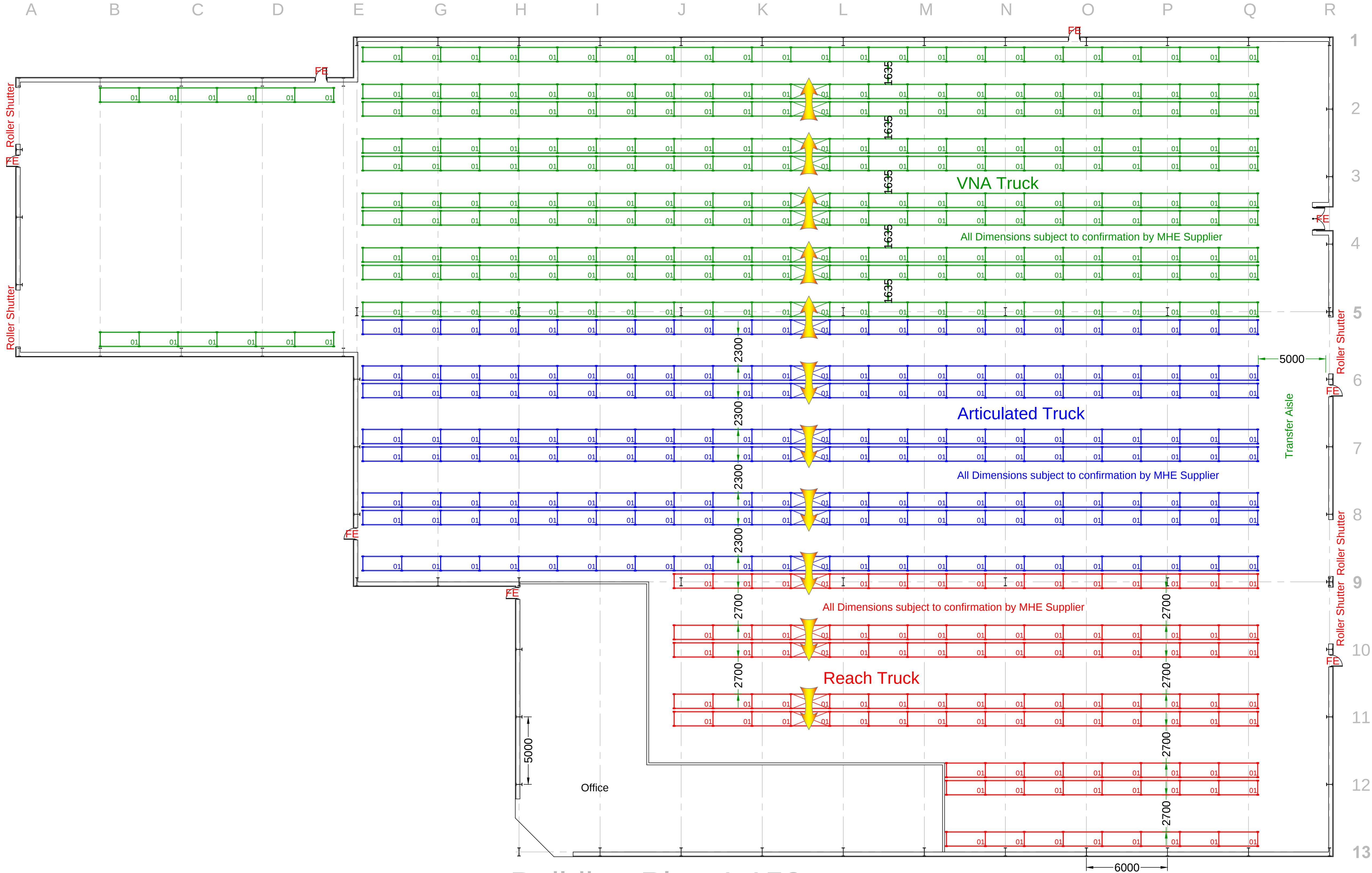
Building Plan 1:150
