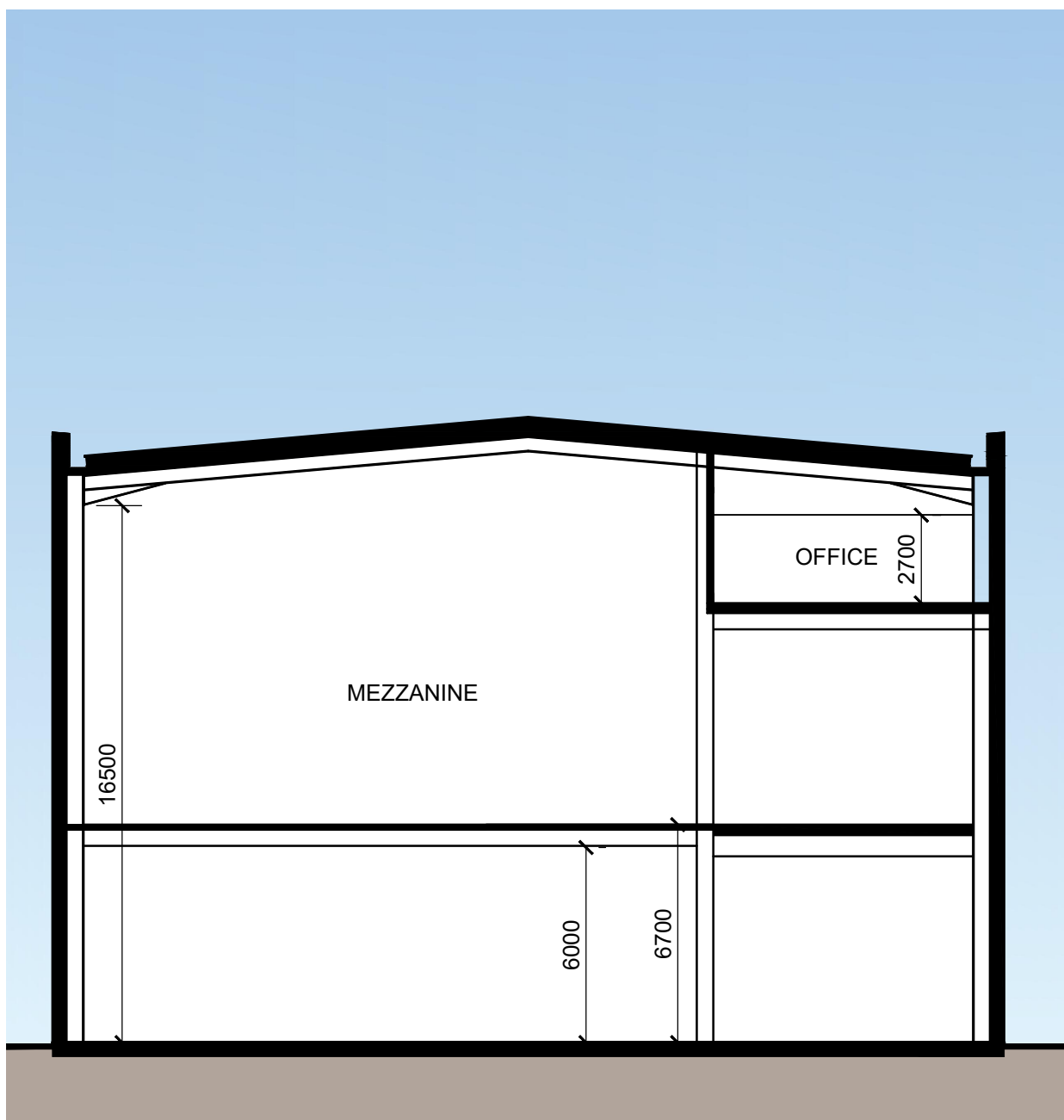
INDICATIVE SECTION
