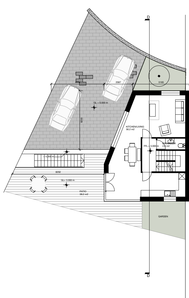
LEVEL 01 PLAN
