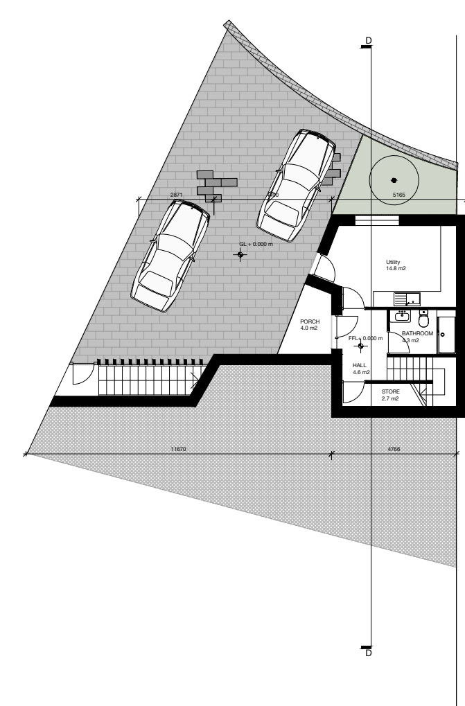
LEVEL 00 PLAN
