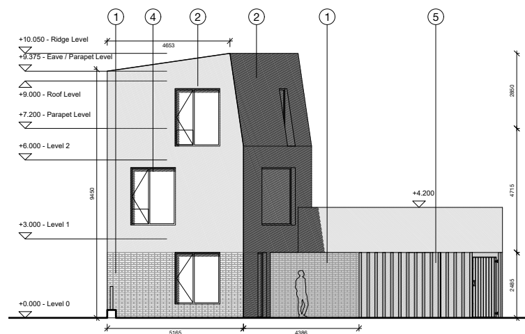
NORTH ELEVATION
