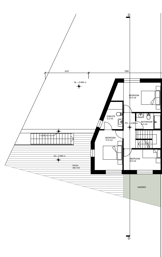
LEVEL 02 PLAN
