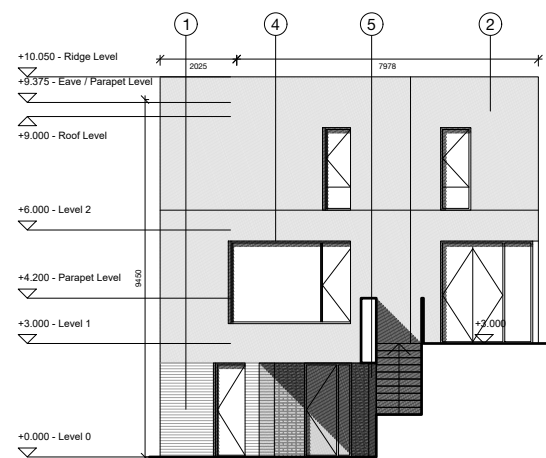
WEST ELEVATION
