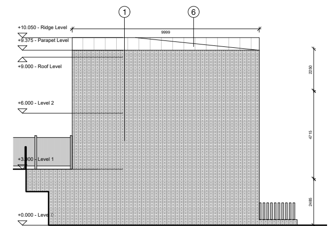
EAST ELEVATION/SECTION
