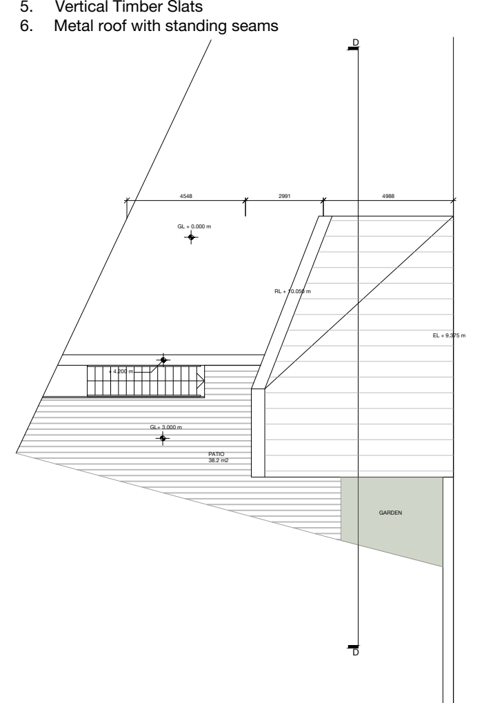
ROOF PLAN
