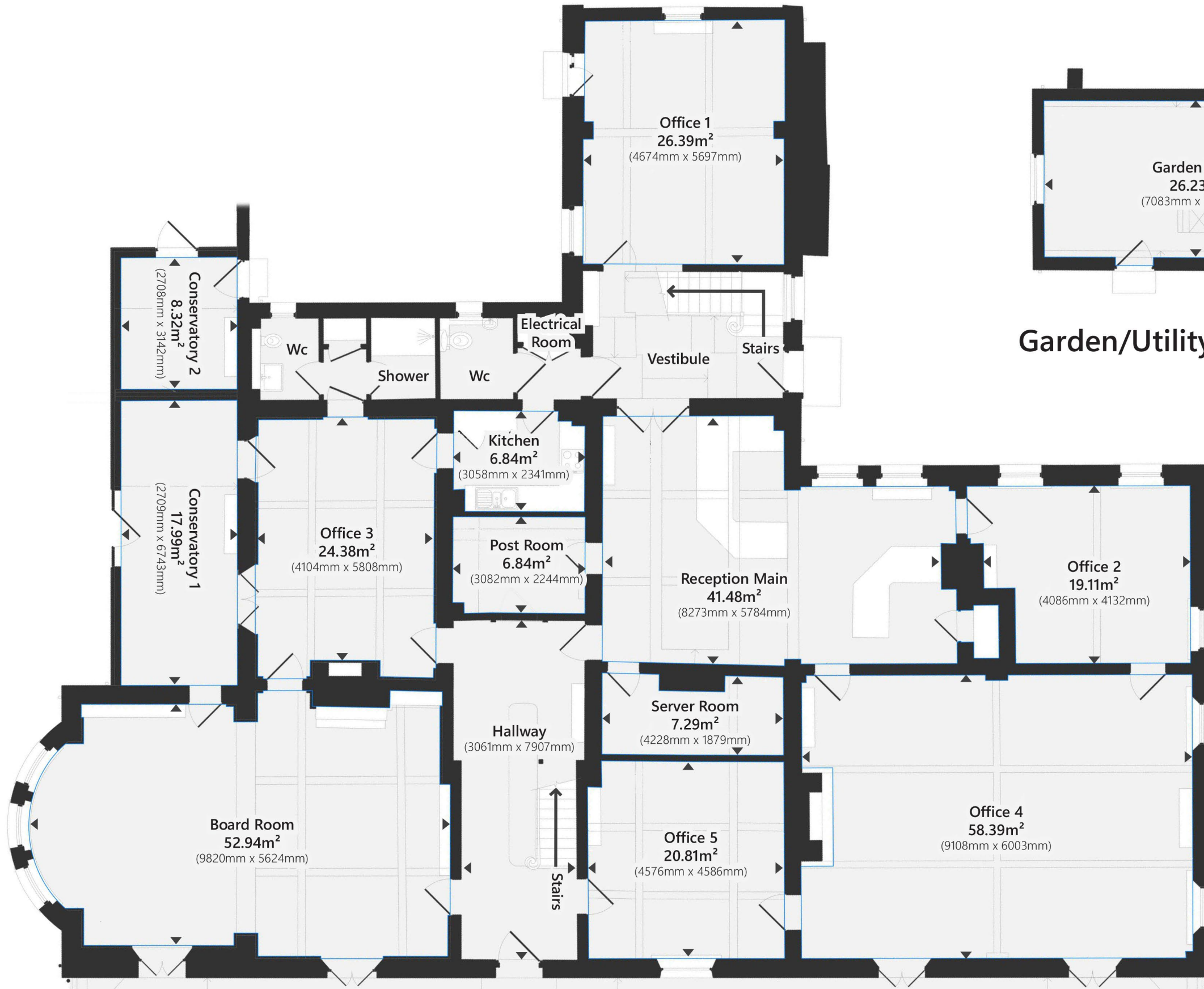
Inhurst House Ground Floor 349m 2
