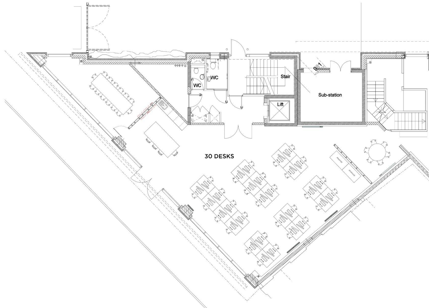
1 GF PLAN (UNIT 1) Scale: 1:50
