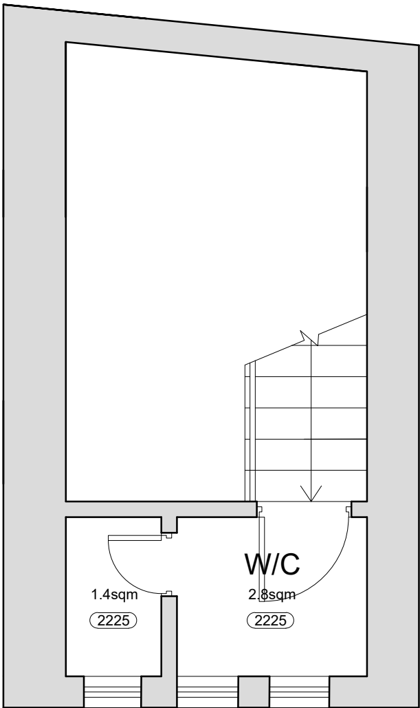
Existing Second Floor Stair Plan Scale: 1:50
