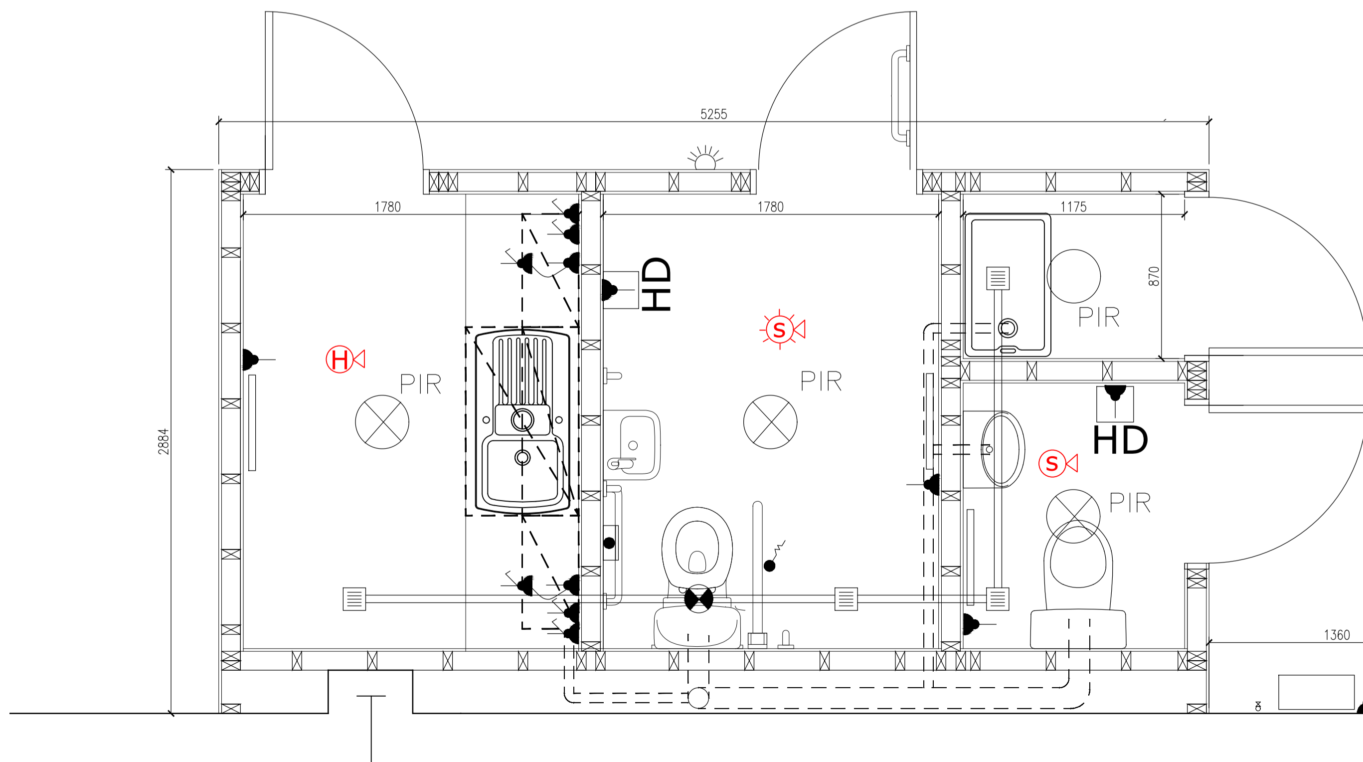
Proposed WC/Kitchenette block 1:20
