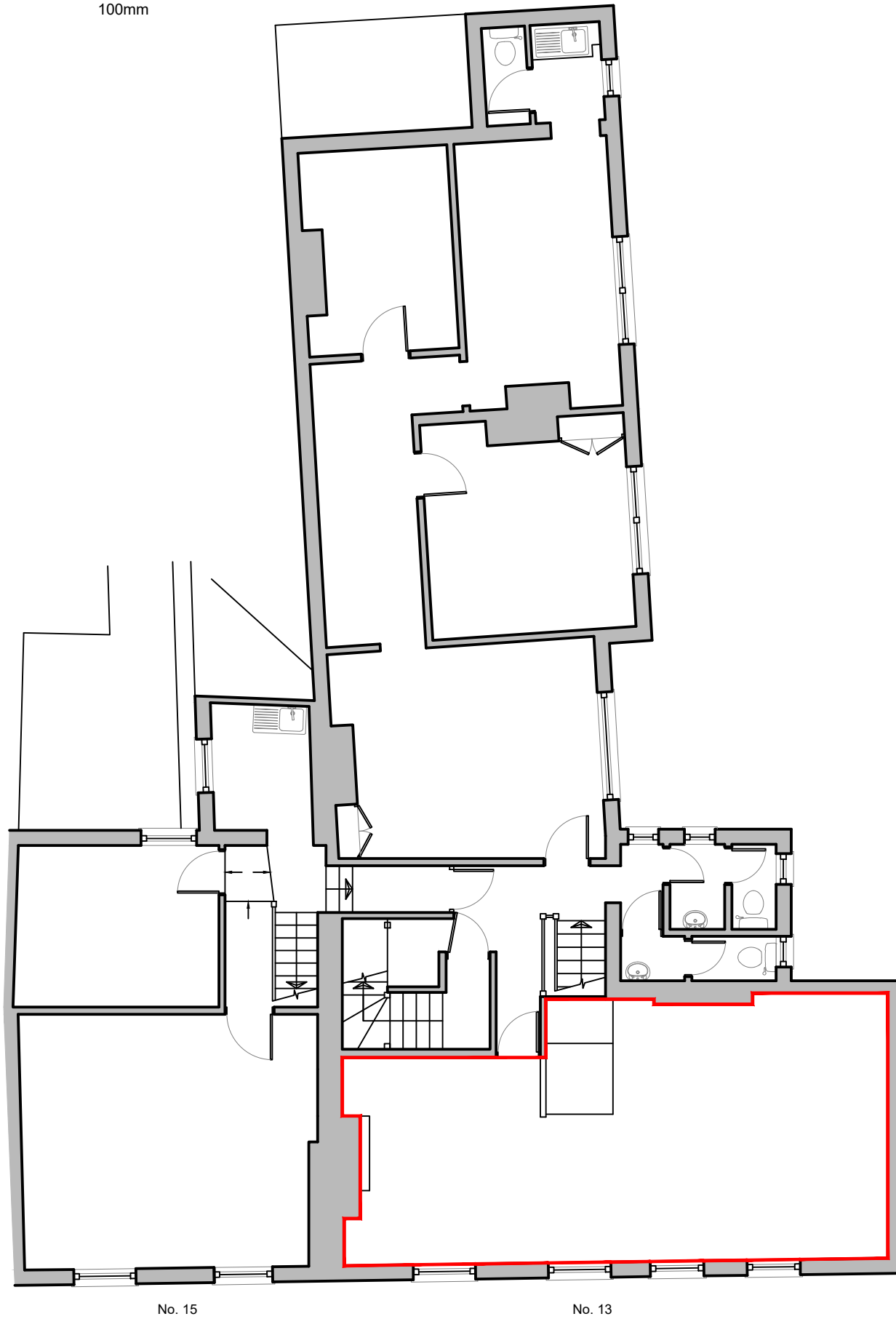
FIRST FLOOR @ 1:100
