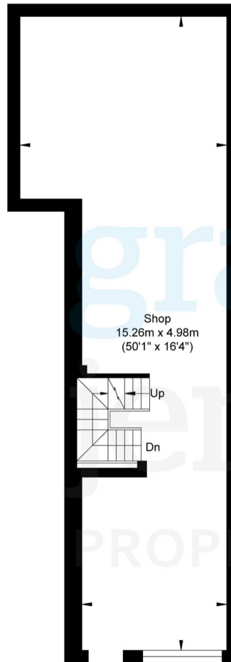
Ground Floor Approximate Floor Area 646.05 sq ft (60.02 sq m)
