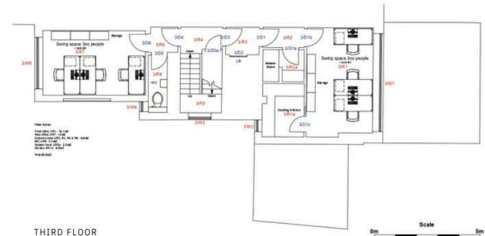
THIRD FLOOR
