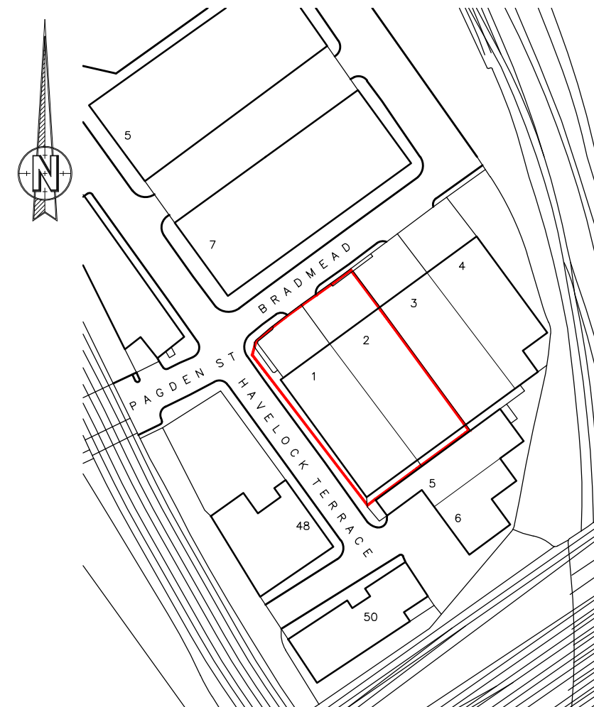
LOCATION PLAN @ 1:1250 0m 10m 20m 30m 40m 50m K.A.D. Licensed O.S. No. 100047482
