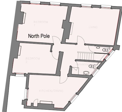
4 Existing Second Floor Plan 1 : 200
