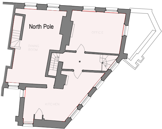
3 Existing First Floor Plan 1 : 200
