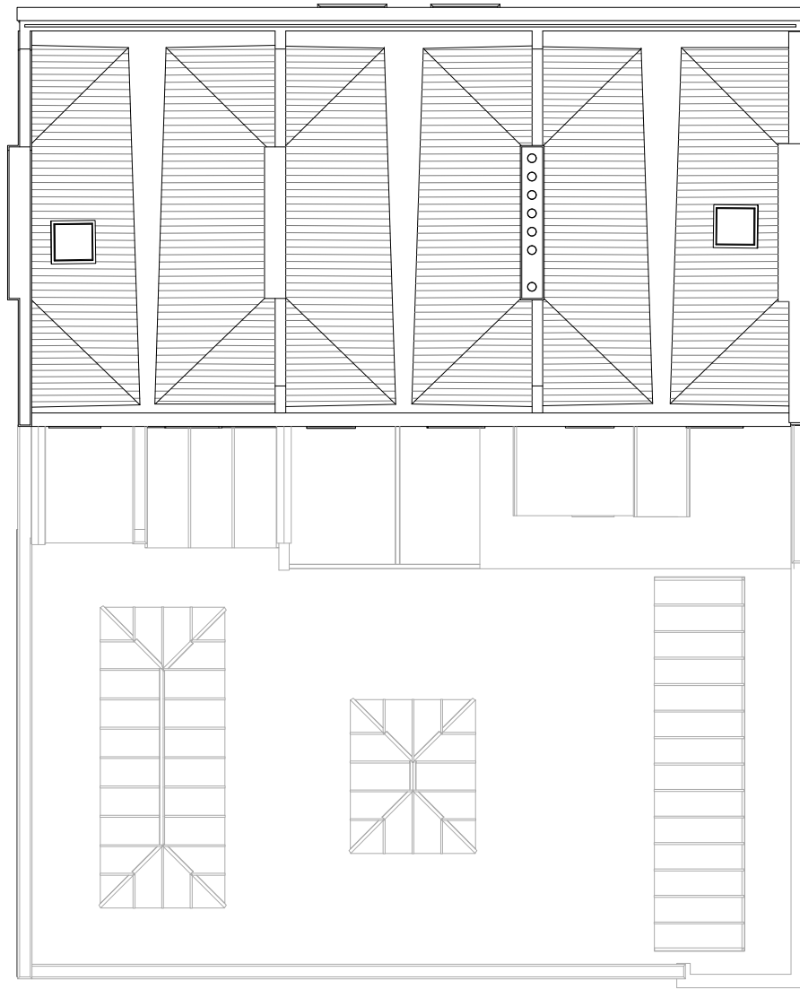
1 Existing Roof Plan 1 : 100
